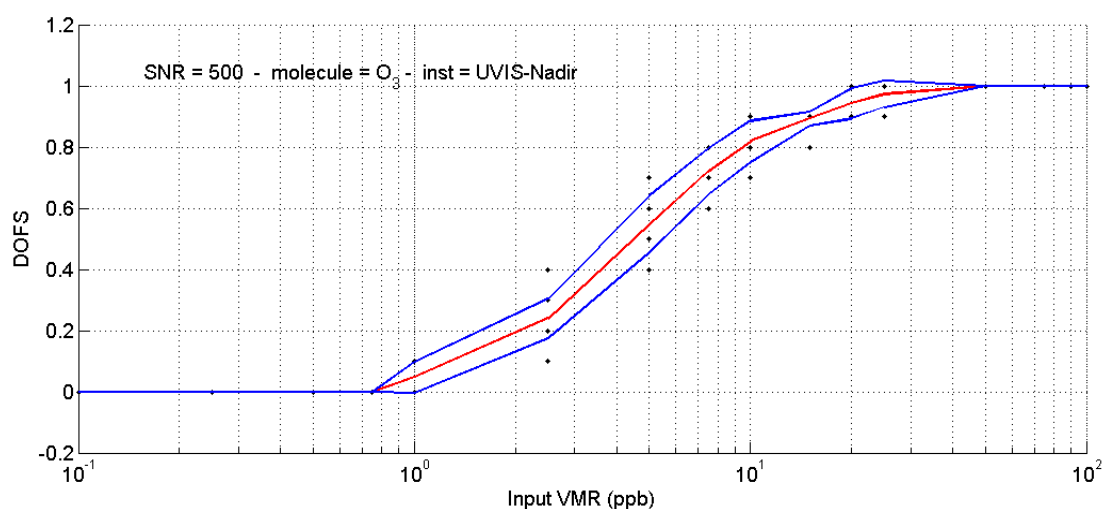
Figure 4: DOFS criterion applied to the O_3 detection. The red curve represents the average DOFS value obtained for a given initial abundance and the blue curves the 2-sigma standard deviation.
