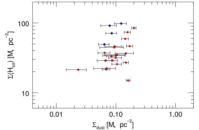
Figure 7. Correlation plot of the mass column densities of classical dust (i.e., excluding PAHs) as inferred from our fits of individual extinction curves, vs. the total mass density of H (atomic and molecular, in all charge states) along the same individual lines of sight. Blue dots are SMC lines of sight, red dots LMC ones.
