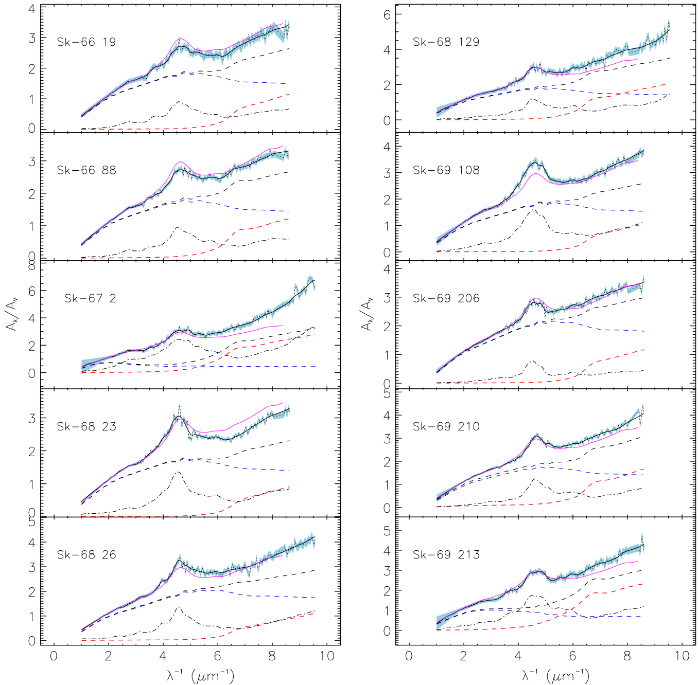
Figure 2. Fits to the normalized extinction curves for lines of sight in the Large Magellanic Cloud. Solid black lines: global fit. Dashed lines: classical dust contribution; in blue the contribution of “large” dust grains, in red “small” dust grains, in black their sum; only the black curve is shown when the gap is very small or nonexistent. Dotted–dashed lines: PAHs. Solid purple line, the “average” extinction curve for the LMC (Gordon et al. 2003). Dotted–dashed lines: PAHs. The lightly shaded areas are the observational error ranges (see text). Fits to the normalized extinction curves for lines of sight in the Large Magellanic Cloud LMC2 Ss. Solid black lines: global fit. Dashed lines: classical dust contribution; in blue the contribution of “large” dust grains, in red “small” dust grains, in black their sum; only the black curve is shown when the gap is very small or nonexistent. Dotted–dashed lines: PAHs. Solid purple line, the “average” extinction curve for the LMC (Gordon et al. 2003). Dotted–dashed lines: PAHs. The lightly shaded areas are the observational error ranges (see text).
