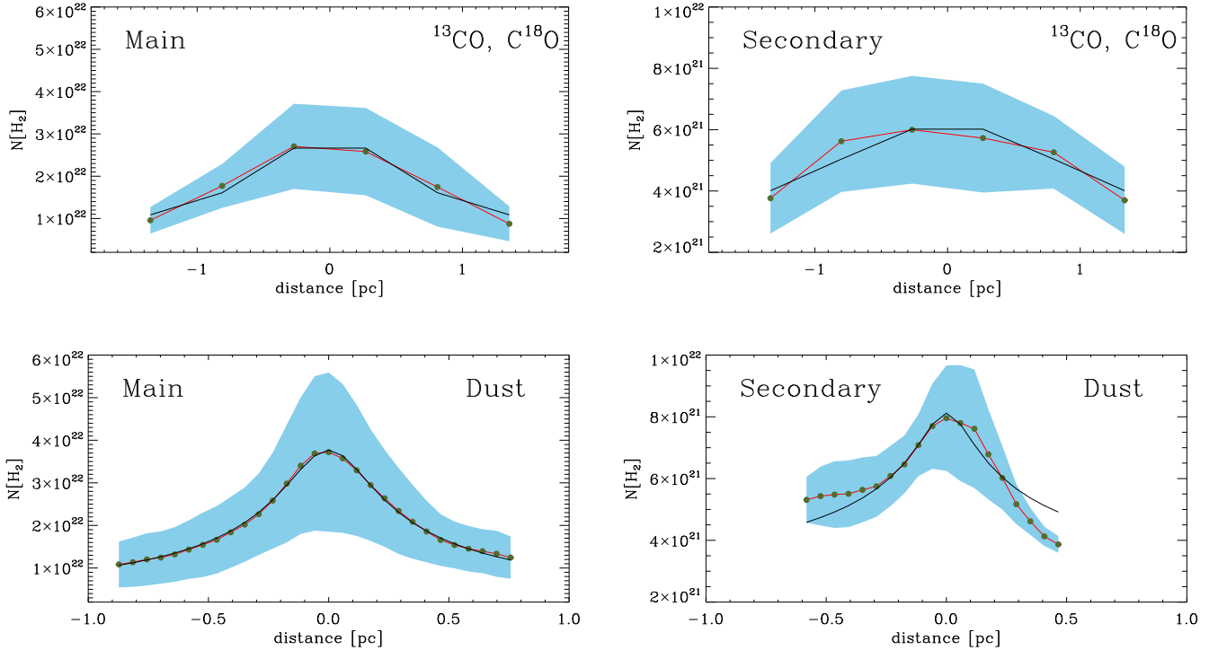
Fig. 11. Radial column density profile of the main ( left column ) and secondary ( right column ) filaments. The dots, connected by the red solid line, show the mean profile across the filaments, while the shaded area indicates the standard deviation. In the top row the average profiles were estimated from the ^{13}\text{CO} and \text{C}^{18}\text{O}(1-0) derived column density (Fig. 5, top panel), while in the bottom row we used the column density estimated by Elia et al. (2013) . The black solid line represents the best fit profile, following the formulation in Arzoumanian et al. (2011) .
