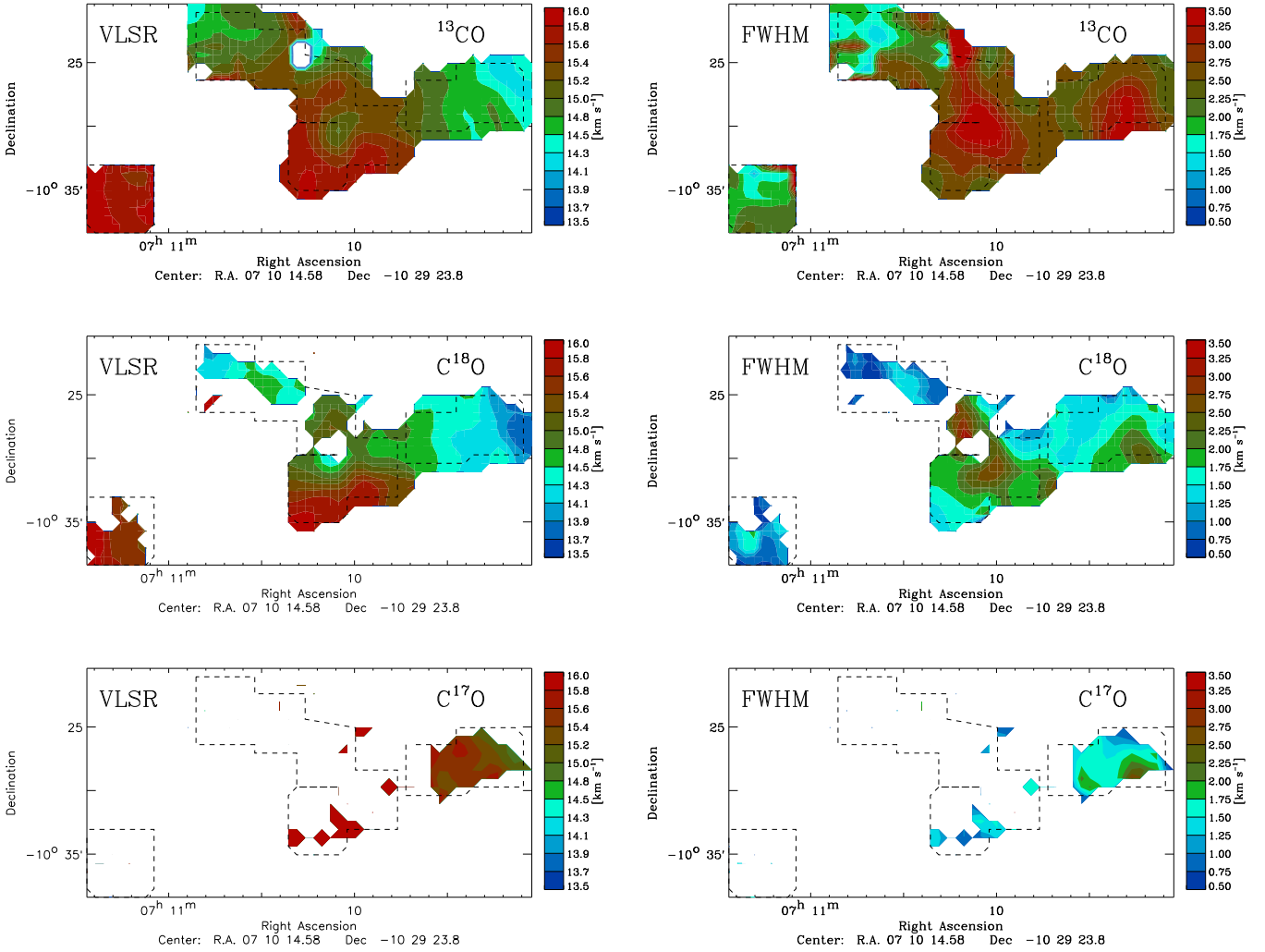
Fig. 8. Line center velocities ( left column ) and line widths ( right column ) after convolving ( from top to bottom ) the ^{13}\text{CO} , \text{C}^{18}\text{O} and \text{C}^{17}\text{O}(1-0) Mopra maps to 80'' and regridding with a 40'' spacing. The smaller red areas are map artifacts.
