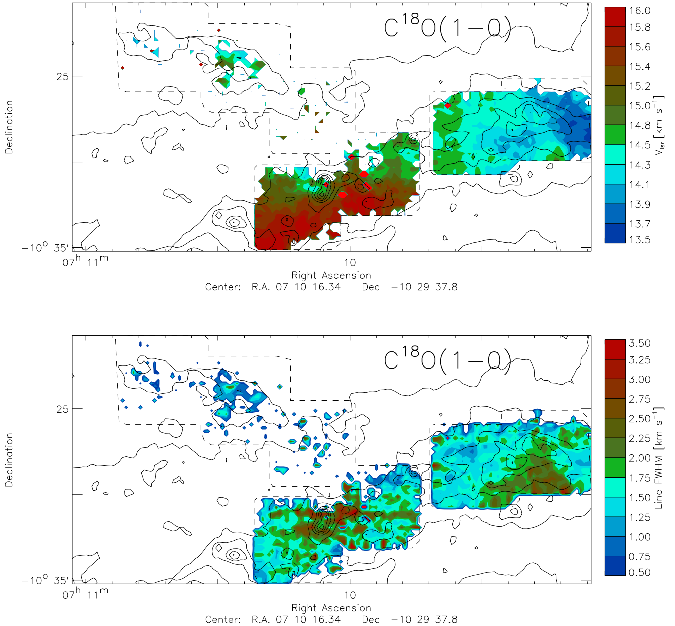
Fig. 7. Same as Fig. 6 for C^{18}O(1-0) . The line centers and line widths have been computed by fitting a 1-component Gaussian to the spectrum at each point (see text).
