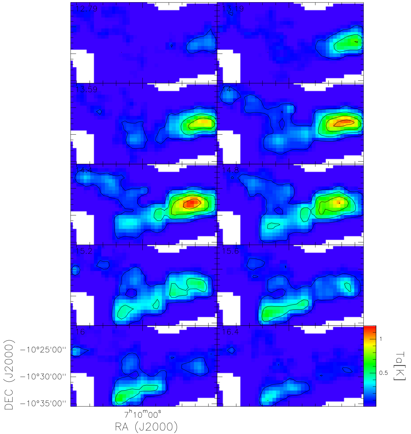
Fig. A.4. Same as Fig. A.3 for C^{18}O(1-0) .
