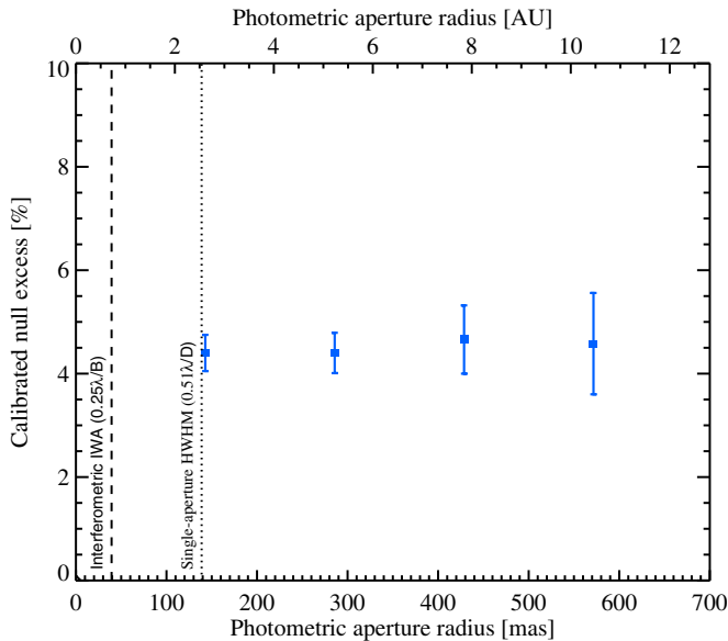
Figure 2. Calibrated null excess as a function of photometric aperture radius. The left vertical dashed line indicates the interferometric inner working angle (i.e., \lambda/4B = 39 mas or 0.7 AU at a distance of \eta Crv), while the right vertical dotted line represents the default aperture radius used in this study (i.e., the HWHM of the single-aperture PSF at 11.1 \mu\text{m} ). The lack of a significant increase in the null measurements for larger aperture radii suggests that the regions emitting a majority of the N' -band flux is more compact than the size of the single-aperture PSF.
