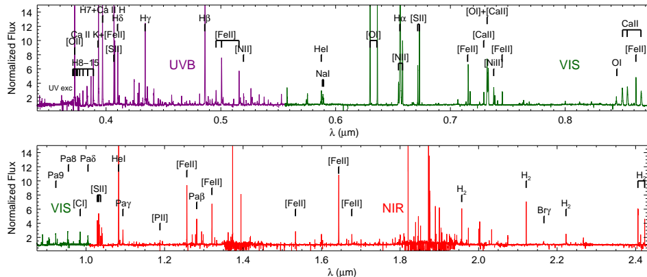
Fig. 1. X-Shooter spectrum of the pre-main sequence object Sz102 (Antoniucci et al., in prep.). The main emission features detected, which trace different structures of the source (see text), are indicated.
