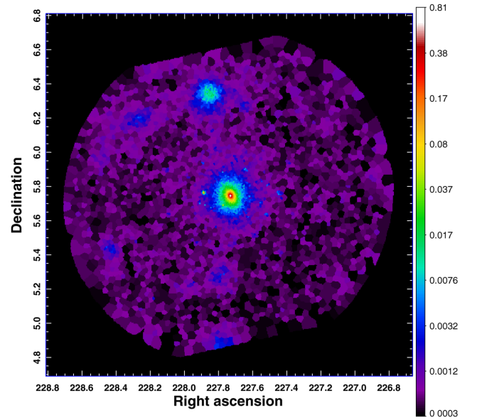
Figure 4. ROSAT/PSPC surface-brightness image of A2029 obtained using Voronoi tessellation (Cappellari & Copin 2003), in units of counts s^{-1} arcmin ^{-2} . Each Voronoi bin includes an average of 20 counts.
