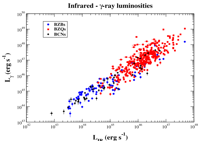
Figure 20. Scatter plot of the infrared- \gamma -ray fluxes (upper panel) and luminosities (lower panel) for the blazar-like sources. Spectroscopically confirmed BZBs and BZQs are shown in blue circles and red squares, respectively, while BCN sources are black diamonds.
