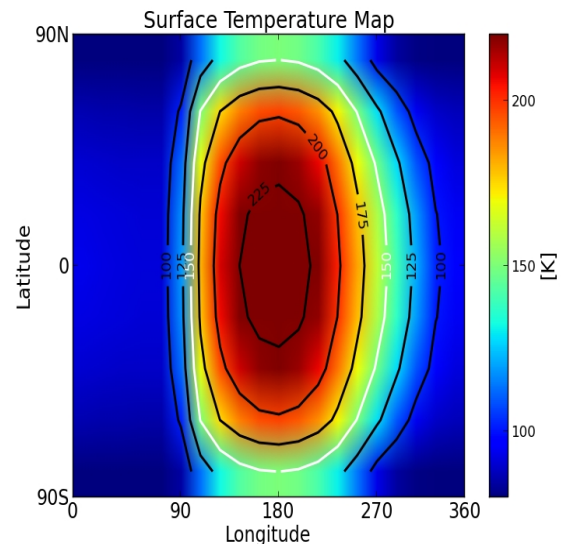
Fig.1: Typical surface temperature. we examined the cases of 163 K, i.e. equilibrium surface temperature assuming a solar constant of 1330 \text{ W m}^{-2} and an emissivity of 0.9, and the case of a lower temperature, i.e. 80 K. The water ice has been considered on the surface or at different distance from the surface: 0.25 m (comparable with the diurnal skin depth of 0.15 m) and 100 m (below the annual skin depth of about 9 m). A typical surface temperature map, in case of silicatic crust (no ice on the surface), is shown in Fig.1.
