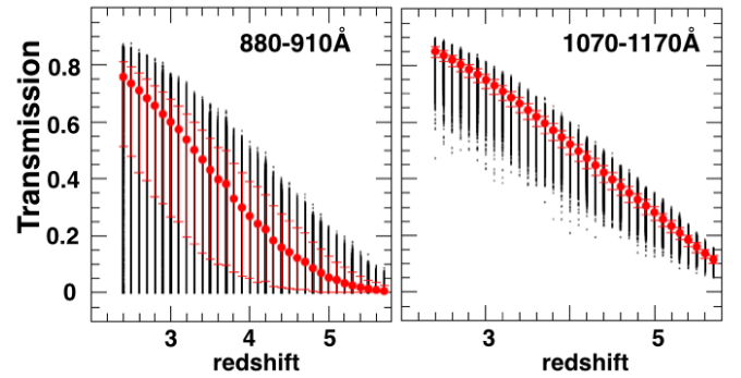
Fig. 2. IGM transmissions as a function of redshift calculated in the wavelength intervals 880–910 Å (left) and 1070–1170 Å (right). At each redshift, 10 000 line of sights have been computed (black points), and the medians with the central 68% intervals are also shown (red filled circles with errorbars).
