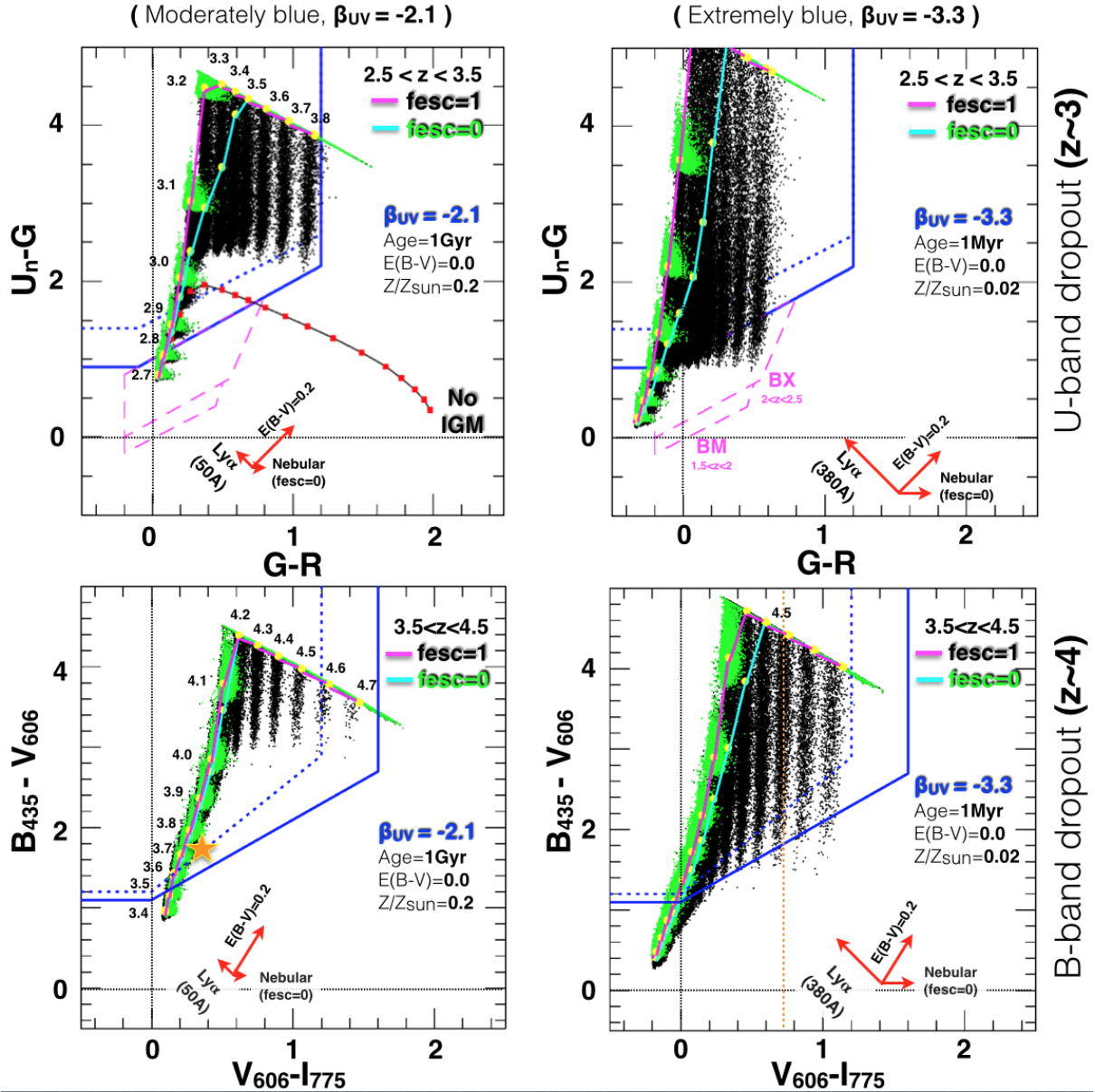
Fig. 3. Top panels: U_nGR color planes with the typical selection regions for galaxies (solid blue line) in the redshift range 2.5 < z < 3.5 are shown for moderately blue (left) and extremely blue (right) galaxy templates. The effect of dust extinction and Ly \alpha emission is shown with red arrows. The green clouds and black stripes correspond to fesc=0 and fesc=1 , respectively, and are computed with redshift steps of 0.1 indicated at the left side. Magenta and cyan solid lines connect the barycenter of each cloud/strip and represent the average color tracks (see text). In the top-left panel the (solid) black color track with filled (red) squares denotes the case in which the IGM is absent from the ionizing part of the spectrum, i.e., the transmission is equal to 1. The rightmost filled square symbol represents z = 4.5 ; squares have been plotted with dz = 0.1 . The color track resembles the behavior of the flat models of Cooke et al. (2014) (see Sect. 3.1). Magenta dashed lines underline the BM and BX selection regions. Bottom panels: same as top panels, but in this case, the BVI ( B_{435}, V_{606}, i_{775} ) color selections of galaxies expected to lie in the redshift range 3.4 < z < 4.5 are shown (solid blue lines). In the bottom-left panel the star indicates the position of the Lyman-continuum emitters Ion1 at z = 3.795 (see text). In the bottom right panel the vertical orange dotted line highlights the bending of the black stripe at z = 4.5 when ionizing emission also affects the V_{606} -band, visible as a slightly bluer V_{606} - i_{775} color for the higher IGM transmission cases (see text). The effect of the LyC leakage on colors decreases with increasing redshift (passing from U-band to B-band dropout selection methods) as a result of redshift evolution of the mean free path of ionizing photons. In all quadrants the triplets of red arrows mark the direction and magnitude of the color modification as a result of the Ly \alpha emission, nebular continuum (affecting only the fesc=0 case, green points), and the dust attenuation, E(B-V) .
