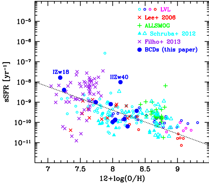
Fig. 6. Specific SFR vs. 12 + \log(\text{O}/\text{H}) for our sample and including data from the literature (Hunt et al. 2012; Schruba et al. 2012; Filho et al. 2013; Bothwell et al. 2014). The metallicities for the ALLSMOG (Bothwell et al. 2014) sample have been modified as discussed in the text. As in Fig. 4, the open triangles for Schruba et al. (2012) correspond to their compilation of data from the literature and the filled ones to their metal-poor dwarf observations. The regression line is a robust best-fit of the Local Volume Legacy (LVL, Lee et al. 2009) and the dwarf irregulars from Lee et al. (2006). The various colors for the LVL give the Hubble type (early types red, magenta; late types blue, cyan).
