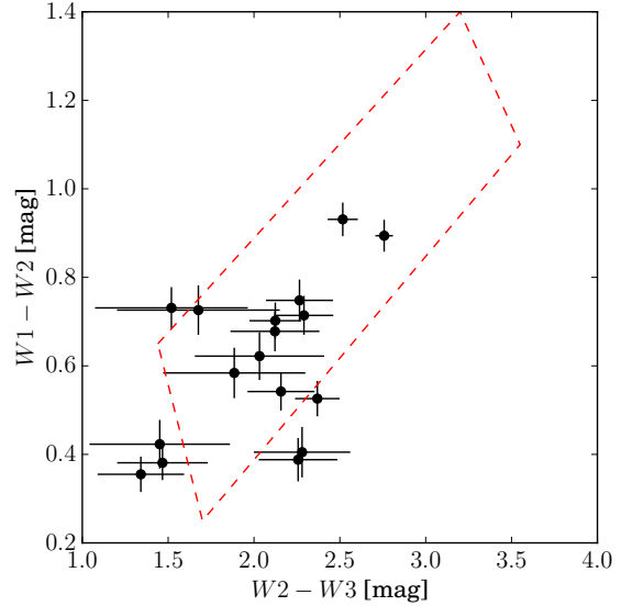
Fig. 7 Plot of the infrared colours of the MST-selected BL Lac objects from the AllWISE catalogue. The dashed line define the region where the WISE Blazar strip is located according to the recent analysis by D’Abrusco et al. (2014). The majority of our sources lie within the strip and those outside the boundaries are generally affected by large errors making possible their location inside the \gamma -ray loud region.
