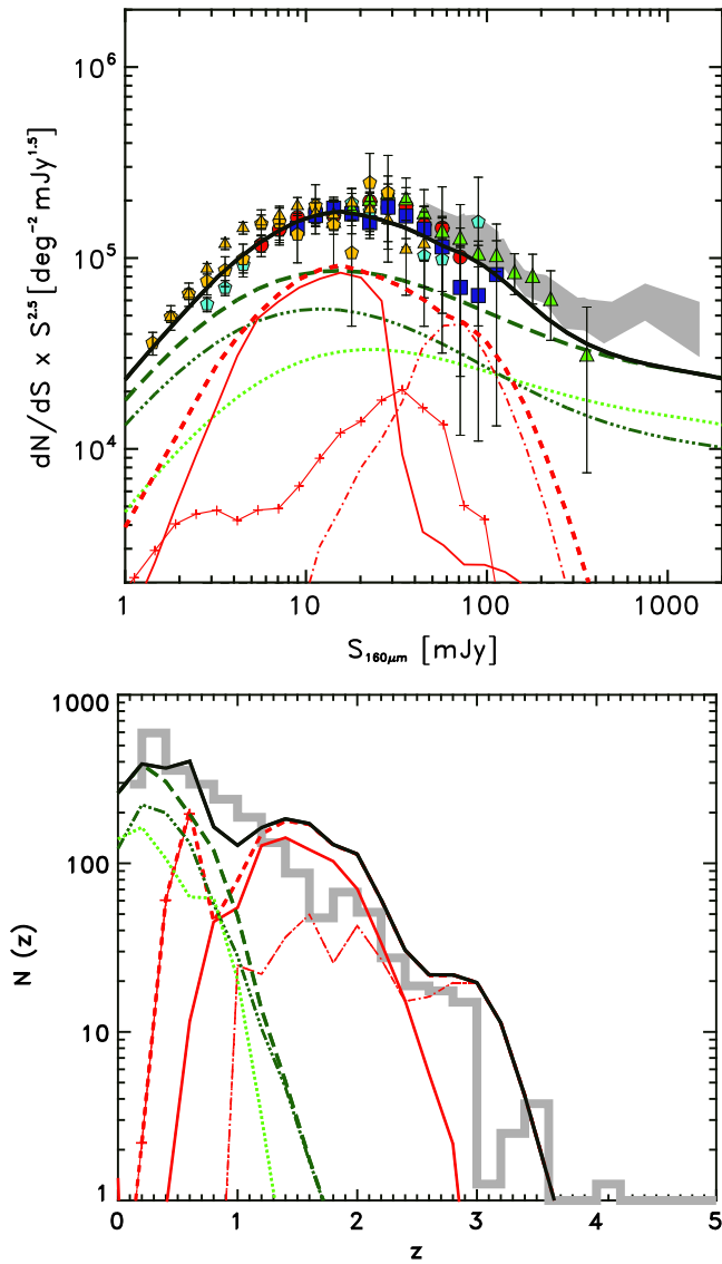
Figure 10. Upper panel: differential extragalactic source counts normalized to the Euclidean slope at 160\ \mu\text{m} . The curves represent the model predictions, calculated by taking into account the downsizing of proto-spheroids. The thin solid line with crosses, the thick solid line, and the dot-dashed line represent the contribution of the proto-spheroid population of present-day stellar mass 3 \times 10^{10} , 10^{10} , and 10^{12}\ M_{\odot} , respectively; the dotted green line represents the spiral, the dot-dot-dot-dashed dark green the SF-AGN (spiral), while the long-dashed dark green the spiral+SF-AGN (spiral) populations. The observational data are as described in the top panel of Figure 3. In the lower panel, the redshift distribution is shown. The curves are as in the top panel and the observational data are as described in the bottom panel of Figure 3.
