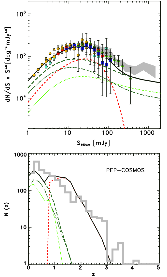
Figure 3. Upper panel: 160\ \mu\text{m} differential extragalactic source counts normalized to the Euclidean slope. Herschel data from PEP (Berta et al. 2011) are represented by red filled circles (GOODS-N), blue filled squares (Lockman Hole), green triangles (COSMOS), and cyan pentagons (GOODS-S). The gray shaded area represents the 1\sigma uncertainty region of the Spitzer data (Dole et al. 2004; Frayer et al. 2006; Béthermin et al. 2010). The Herschel data from the combined PEP/GOODS-H map (Magnelli et al. 2013) are represented by yellow dots (GOODS-S ultra-deep) and yellow pentagons (GOODS-N/S deep). Lower panel: Redshift distribution of the PEP sources with 160\ \mu\text{m} flux > 20 mJy (gray histogram, bin = 0.2). The model curves for the different populations are plotted in different colors (black solid: total; dotted green: spiral; dot-dot-dot-dashed dark green: SF-AGN (spiral), long-dashed dark green: spiral+SF-AGN (spiral); dashed red: proto-spheroids). For the model results, a piecewise-constant continuous formation for proto-spheroids has been assumed as described in Section 3.2.
