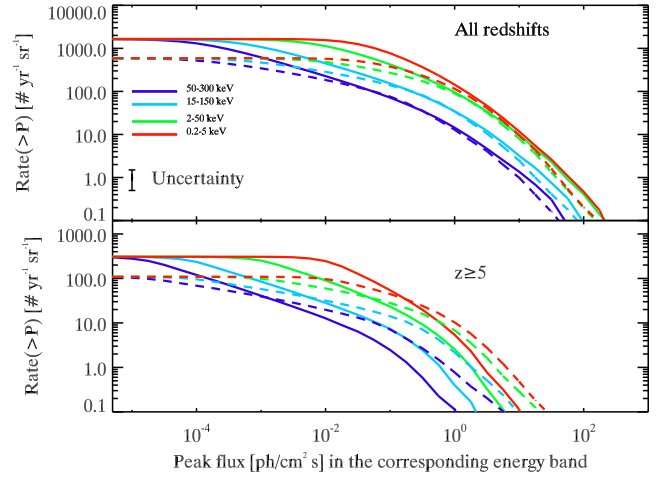
Figure A3. Cumulative distributions of the peak flux comparing the results obtained assuming the evolution of the GRB formation rate (solid lines – Section 2) and the evolution of the LF (dashed lines). Same lines and colour coding of Fig. 4.
