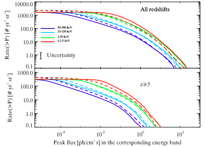
Figure A4. Cumulative distributions of the peak flux comparing the results obtained with the assumptions of Section 2 (solid lines) and that the E_{\text{peak}}-E_{\text{iso}} and E_{\text{peak}}-L_{\text{iso}} correlations are boundaries in the corresponding planes (dashed lines). Same lines and colour coding of Fig. 4.
