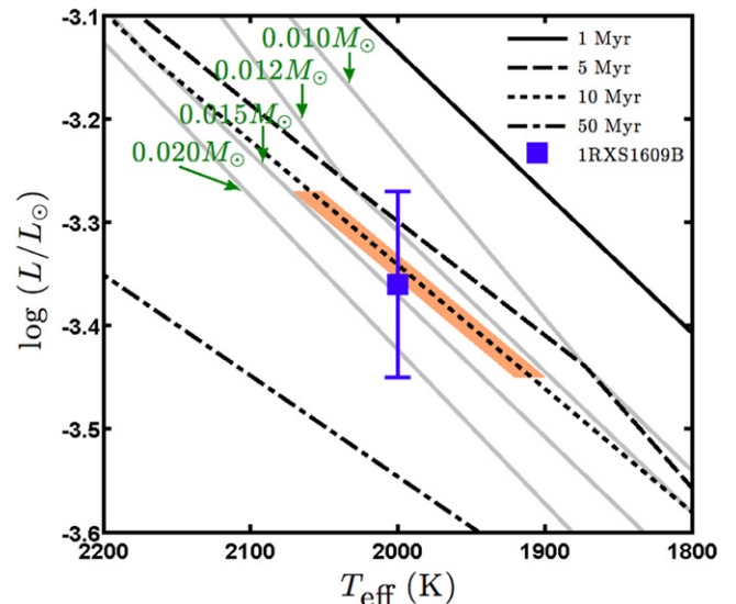
Figure 4. H–R diagram with DUSTY evolutionary tracks. Iso-mass curves are shown in gray. The salmon colored polygon is the only region consistent with the observed T_{\text{eff}} = 1900 – 2100 K, \log(L_{\text{bol}}/L_\odot) = -3.36 \pm 0.09 , and the age of Upper Sco ( 11 \pm 2 Myr). This yields a mass estimate of 0.012 – 0.015 M_\odot .
