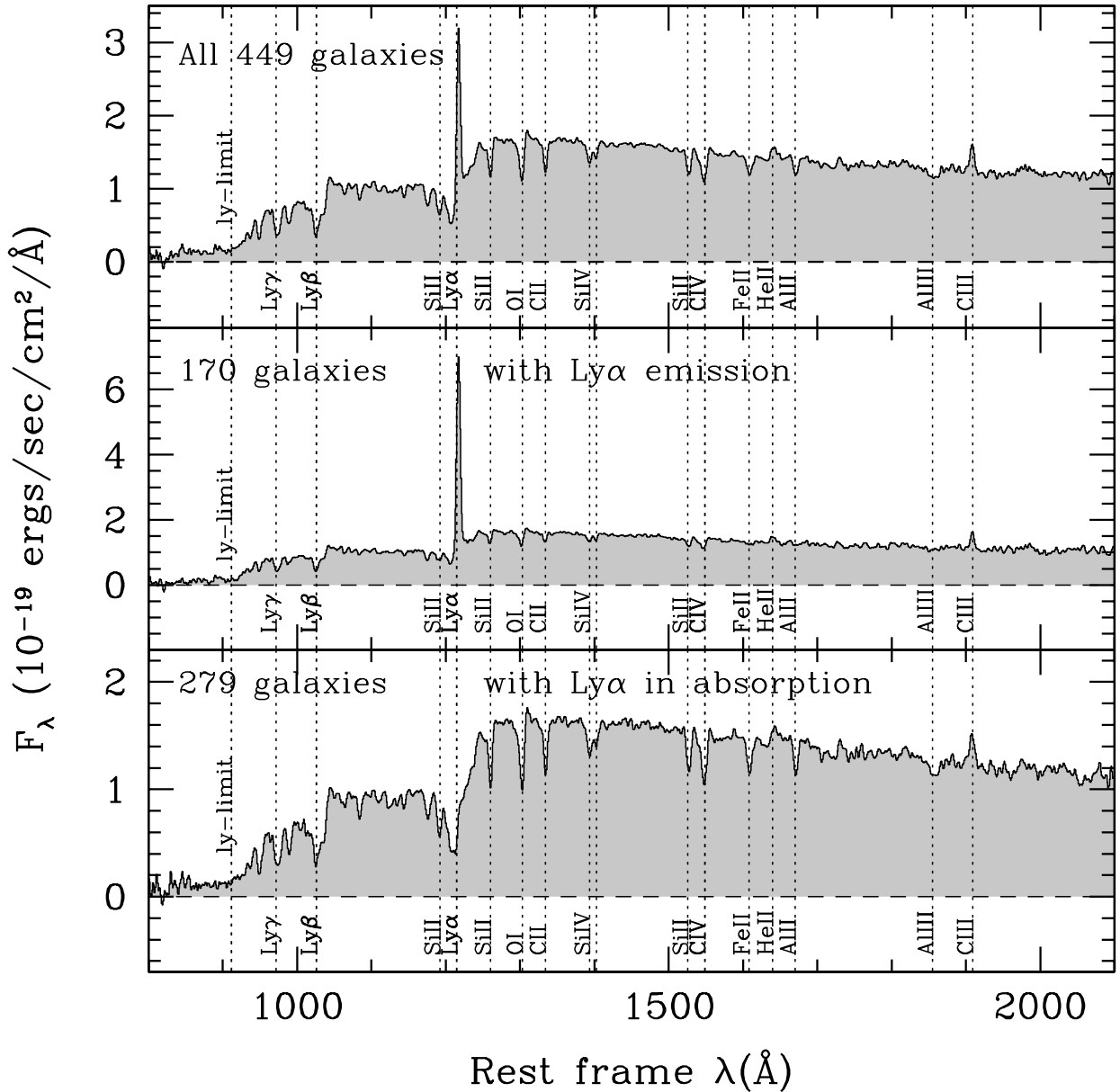
Fig. 20. Average rest-frame spectra ( F_\lambda ) of galaxies with flags 3 and 4 in VUDS with 3 < z < 4 : top : stack of all galaxy spectra; middle : stack of galaxies with Ly- \alpha in emission; bottom : stack of galaxies with Ly- \alpha in absorption (this stack is from a subset of the final sample available at the time of writing).
