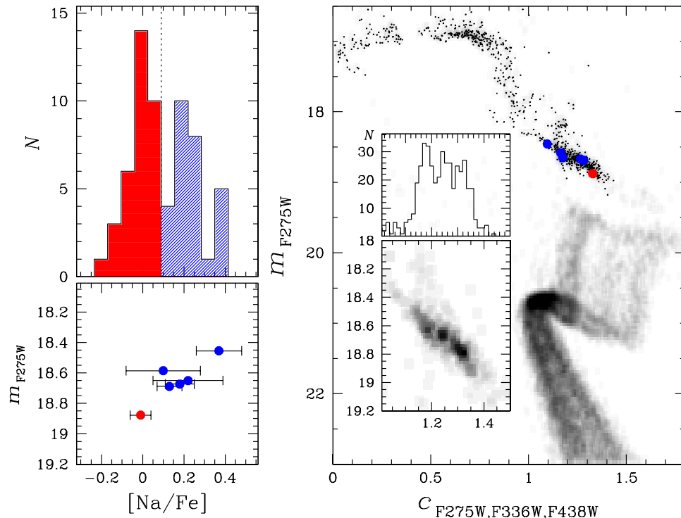
Figure 18. Upper-left panel: histogram of the distribution of [\text{Na}/\text{Fe}] for red HB stars (Marino et al. 2014). Lower-left panel: m_{F275W} vs. [\text{Na}/\text{Fe}] . Right panel: m_{F275W} vs. C_{F275W,F336W,F438W} Hess diagram. The Hess diagram in the inset is a zoom around the red HB, and the histogram of the distribution in C_{F275W,F336W,F438W} for red HB stars is also shown. Na-rich and Na-poor stars defined by Marino and collaborators are colored blue and red, respectively.
