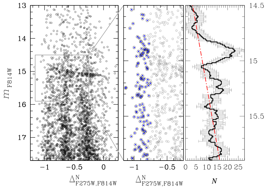
Figure 16. Left panel: reproduction of the m_{\text{F814W}} vs. \Delta_{\text{F275W,F814W}}^N diagram for RGB stars of Figure 2. Middle panel: zoom of left-panel diagram around the bump of population E, where RGB-E stars are marked with blue dots. Right panel: histogram of the F814W magnitude distribution. Gray error bars are Poisson errors while the red dashed-dotted line is the assumed luminosity function for the RGB (see text for details).
