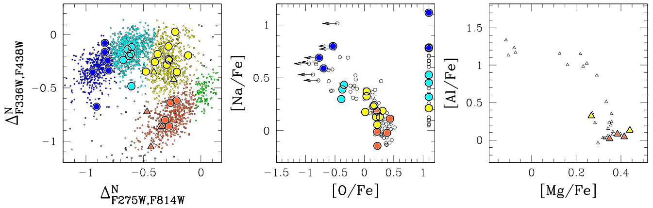
Figure 8. Left panel: reproduction of the \Delta_{F336W,F438W}^N vs. \Delta_{F275W,F814W}^N diagram of Figure 3. Stars for which spectroscopic measurements are available are marked with large symbols. Middle panel: sodium–oxygen anticorrelation for RGB stars of NGC 2808 from Carretta et al. (2006). Large orange, yellow, cyan, and blue dots indicate spectroscopic targets of populations B, C, D, and E, respectively. Stars for which only [Na/Fe] measurements are available have been arbitrarily plotted at [O/Fe] = 1.1. No population-A stars are present in the Carretta et al. sample. Right panel: magnesium–aluminum anticorrelation from Carretta (2014). Population-B and population-C stars are indicated with orange and yellow triangles, respectively.
