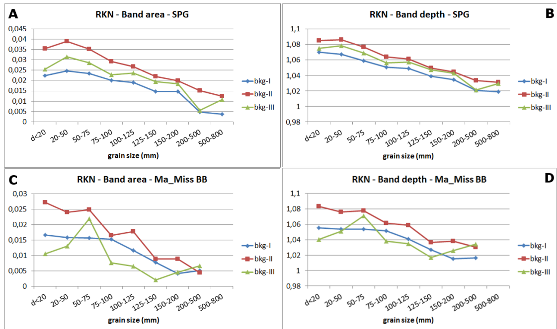
Figure 6. Sample RKN. A and C: band area at 1 \mu\text{m} computed from SPG and Ma_Miss data, respectively, using three different polynomials as continuum background (straight line (I), parabolic (II) and cubic (III)). B and D: band depth at 1 \mu\text{m} computed from SPG and Ma_Miss data, respectively, using three different polynomials as continuum background.
