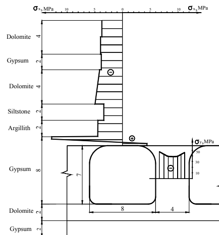
Figure 3. Design Diagram and Stress Epures in Roof and Pillar Rooms.
