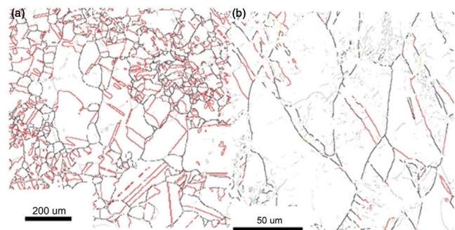
Figure 8. EBSD images of nickel a) before and b) after tension. The density of twins (marked in red) decreases from 38.6% for the virgin sample to 2.47% near the breaking point.
