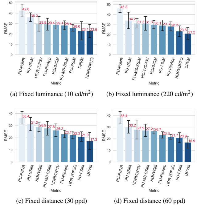
Figure 6: Five-fold cross-validation results for the compared metrics under varied viewing conditions. We fix one of the viewing conditions and make the metric account for the remaining condition. In the first row we isolate distance as the component impacting the VLT and test whether metrics can take it into account under fixed display luminance. Similarly, in the second row, we fix the distance, and let the metrics account for the display luminance. Error bars show the standard deviation.
