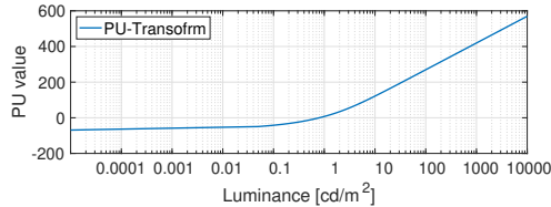
Figure 5: PU-transform used to transform absolute physical values (in cd/m 2 ) into approximately perceptually uniform units that can be used with existing quality metrics. Note, some values are negative – to ensure that the luminance range of a typical (sRGB) monitor of 1 cd/m 2 to 80 cd/m 2 is mapped to the range 0–255.
