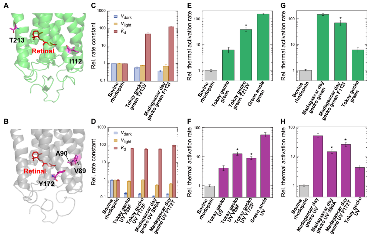
Fig. 3. Key amino acid residues regulate the thermal activation rates ( k_{th} ) of gecko green- and UV-sensitive cone pigments. (A and B) Homology model structures of tokay gecko green (A) and tokay gecko UV (B) that were constructed on the basis of the crystal structure of the dark state of bovine rhodopsin (Protein Data Bank: 1U19). The mutated residues (Val 89 , Ala 90 , Ile 112 , Tyr 172 , and Thr 213 ) and 11-cis-retinal are colored magenta and red, respectively. (C) Comparison of v_{dark} , v_{light} , and k_d of bovine rhodopsin, T213V mutant of tokay gecko green, and F112I mutant of Madagascar day gecko green measured by the biochemical and fluorescence assays (figs. S2 to S4). (D) Comparison of v_{dark} , v_{light} , and k_d of bovine rhodopsin, V89F and Y172F mutants of tokay gecko UV, and S90A and F172Y mutants of Madagascar day gecko UV measured by the biochemical and fluorescence assays (figs. S2 to S4). (E) Comparison of the thermal activation rates ( k_{th} ) of bovine rhodopsin, wild type and T213V mutant of tokay gecko green, and green anole green estimated from the data in (C). (F) Comparison of the thermal activation rates ( k_{th} ) of bovine rhodopsin, wild type and V89F and Y172F mutants of tokay gecko UV, and green anole UV estimated from the data in (D). (G) Comparison of the thermal activation rates ( k_{th} ) of bovine rhodopsin, wild type and F112I mutant of Madagascar day gecko green, and tokay gecko green estimated from the data in (C). (H) Comparison of the thermal activation rates ( k_{th} ) of bovine rhodopsin, wild type and S90A and F172Y mutants of Madagascar day gecko UV, and tokay gecko UV estimated from the data in (D). All error bars represent the SEM of more than three independent measurements. * indicates a significant difference in relative rate constants between the mutants and wild type of tokay gecko green in (E) (Bonferroni, P < 0.05/4 ; ANOVA), tokay gecko UV in (F) (Bonferroni, P < 0.05/5 ; ANOVA), Madagascar day gecko green in (G) (Bonferroni, P < 0.05/4 ; ANOVA), or Madagascar day gecko UV in (H) (Bonferroni, P < 0.05/5 ; ANOVA).
