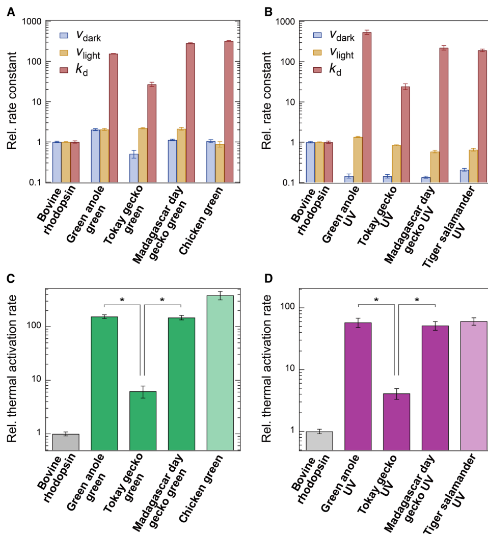
Fig. 2. Comparison of the thermal activation rates ( k_{\text{th}} ) of wild-type gecko visual pigments. (A) Comparison of V_{\text{dark}} , V_{\text{light}} , and k_d of bovine rhodopsin, green anole green, tokay gecko green, Madagascar day gecko green, and chicken green measured by the biochemical and fluorescence assays (figs. S2 to S4). (B) Comparison of V_{\text{dark}} , V_{\text{light}} , and k_d of bovine rhodopsin, green anole UV, tokay gecko UV, Madagascar day gecko UV, and tiger salamander UV measured by the biochemical and fluorescence assays (figs. S2 to S4). (C) Comparison of the thermal activation rates ( k_{\text{th}} ) of bovine rhodopsin, green anole, tokay gecko, Madagascar day gecko, and chicken green estimated from the data presented in (A). (D) Comparison of the thermal activation rates ( k_{\text{th}} ) of bovine rhodopsin, green anole, tokay gecko, Madagascar day gecko, and tiger salamander UV estimated from the data presented in (B). All error bars represent the SEM of more than three independent measurements. * indicates a significant difference in relative rate constants between visual pigments [Bonferroni, P < 0.05/5 ; analysis of variance (ANOVA)].
