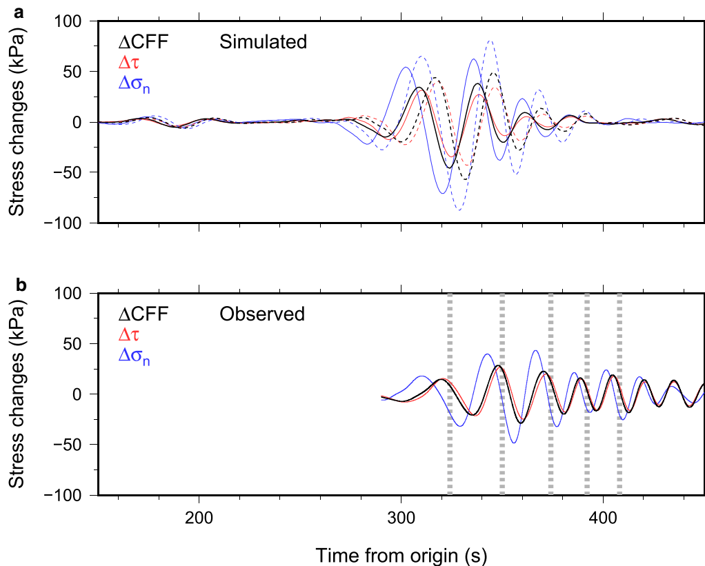
Fig. 4 Stress changes resolved for a mechanism of tremor. \Delta\sigma_n represents the normal stress change, \Delta\tau is the shear stress change in the slip direction, and \Delta CFF is the Coulomb failure function change for the shear slip on the plate interface. a Simulated values at the location estimated by the median epicenter of background tremors are shown as solid lines, and those at the location close to CJIG are shown as dotted lines. b Values at a depth of 45 km estimated from the recorded waveforms beneath station CJIG. The vertical dashed lines in gray correspond to the large peaks of triggered tremors shown in Fig. 2
