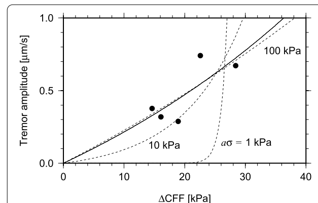
Fig. 5 Relationship between the peak velocity amplitude of the triggered tremor and the peak Coulomb failure stress changes. The solid line represents the regression fit with \alpha\sigma = 56.84 kPa and dotted lines represent the theoretical relationship for \alpha\sigma = 1, 10, and 100 kPa
