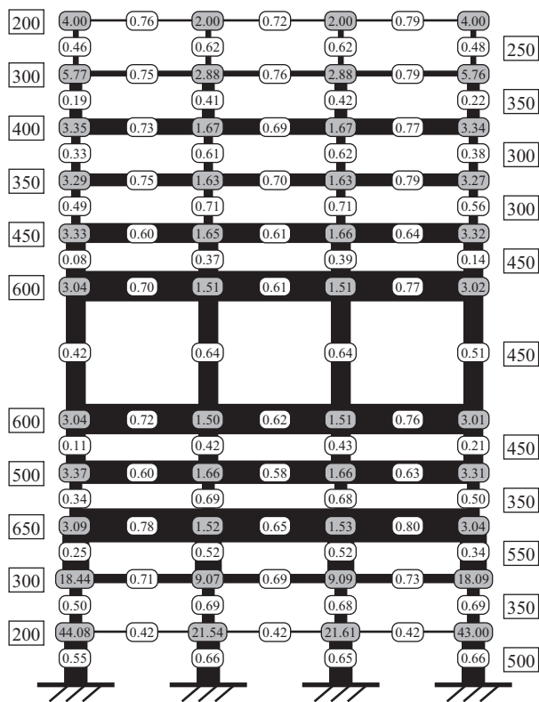
Fig. 14 The best solution of the eleven-story frame obtained by the proposed method ( V = 9.775 \text{ [m}^3\text{]} ).
