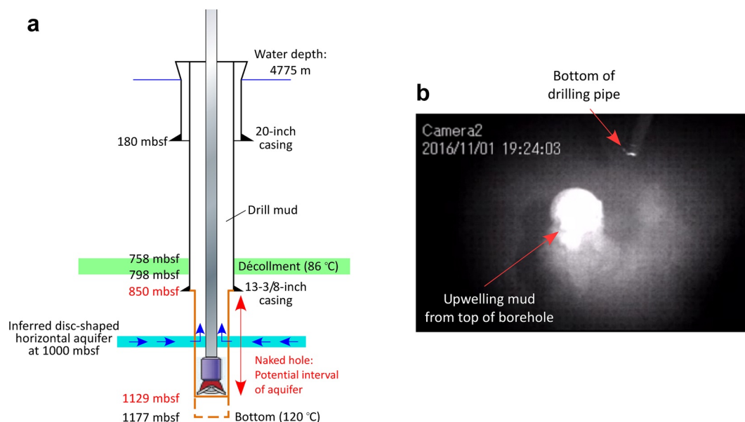
Figure 3. (a) Borehole configuration of Hole C0023 when upwelling flow of drilling mud was observed. For modeling of pore fluid pressure and flow rate, a horizontal disk-shaped aquifer at 1,000 mbsf was assumed. (b) An image of the upwelling mud flow from the well head of Hole C0023 on November 1, 2016 (see also Movie S1).
