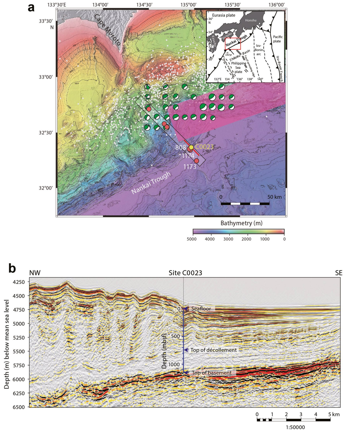
Figure 1. (a) Regional bathymetric map of the area around the drilling site (modified from Heuer et al., 2017) showing locations of Site C0023 (yellow) and nearby Ocean Drilling Program drill sites (red). Black rectangle delineates area of a 3-D seismic survey along the Muroto Transect (Moore et al., 2001). White dots are the epicenter locations of very low frequency earthquakes (VLFs) observed between 2003 and 2018 (Asano et al., 2008; Nakano et al., 2018). Plotted focal mechanisms are the solutions of the largest magnitude VLFE between 2003 and 2018 (compiled from Takemura et al., 2019). The pink shaded rectangle is the estimated area of the 2017–2018 slow slip event (Yokota & Ishikawa, 2020). Inset: Simplified plate tectonics of the area southeast of the Japanese Islands. (b) Prestack seismic depth migration section through Site C0023 (shown by the red line in (a)). Vertical blue line shows the trace of drill hole C0023 with depth scale in meters below seafloor (mbsf); the horizons interpreted to represent the seafloor, top of décollement zone and top of oceanic basement, are labeled.
