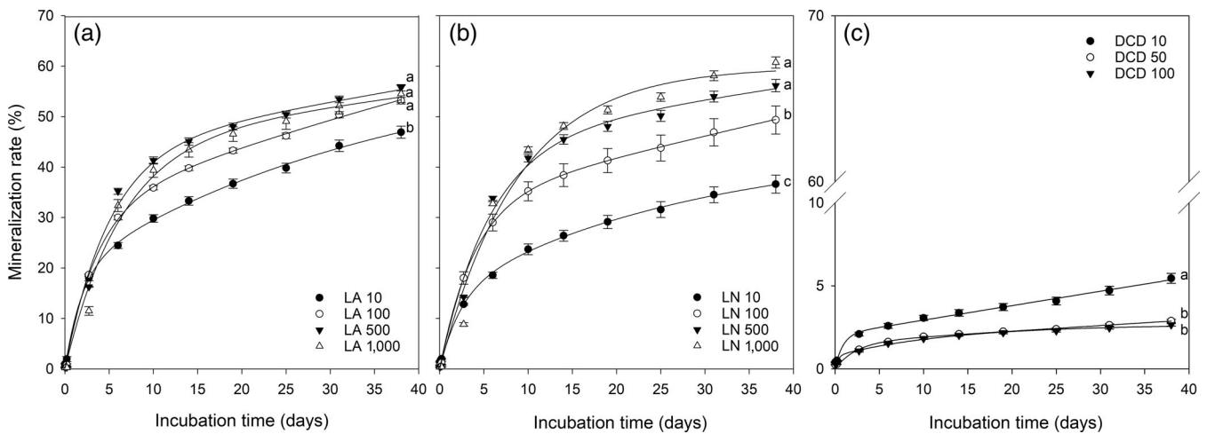
FIGURE 4 Effect of nitrification inhibitor concentrations on mineralization rate of ^{14}\text{C} -labelled linoleic acid (LA, panel (a)), linolenic acid (LN, panel (b)) and dicyandiamide (DCD) (panel (c)) in a sandy clay loam soil during a 38-day incubation at 10^\circ\text{C} . Error bars represent standard error of the mean ( n = 4 ). Different letters indicate significant differences between treatments at p < 0.05 by LSD test
