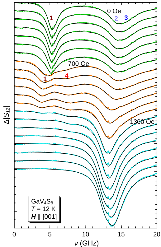
Figure 6. Broadband microwave transmission spectra |S_{12}| of \text{GaV}_4\text{S}_8 taken at T = 12\text{ K} for different magnetic fields applied along the cubic [001] direction in Cyc (green), SkL (orange), and FM (blue) phases. Black solid lines represent fits by Lorentzian lines as described in the text.
