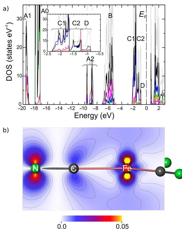
Figure 4. a) DOS for \text{LiSr}_3[\text{Fe}(\text{CN})_3] (total DOS gray, muffin-tin part black, Li partial DOS (pDOS) cyan, Sr pDOS green, Fe pDOS blue, C orange, and N magenta). Inset shows detailed view on DOS regions C (composed of C1 and C2) and D indicating slight overlap between C2 and D, where vertical red line marks boundary between nominal C1 + C2 (10 e/f.u.) and D (4 e/f.u.) regions. b) Electron density calculated for electronic states from upper part of DOS region D with 1.74 e/f.u. See text for further details.
