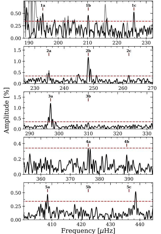
Figure 5. Possible evidence for five \ell = 1 mode splittings, identified within the GD 278 TESS periodogram and listed in Table 2 . Red tick marks indicate the frequencies that we propose form rotationally split multiplets, consistent with an overall 10 hr rotation rate. For each mode we show in grey the prewhitened TESS light curve, subtracted of all frequencies listed in Table 1 other than those indicated by the red points, and show the resulting periodogram in black. The red dashed lines mark the 0.34% significance threshold.
