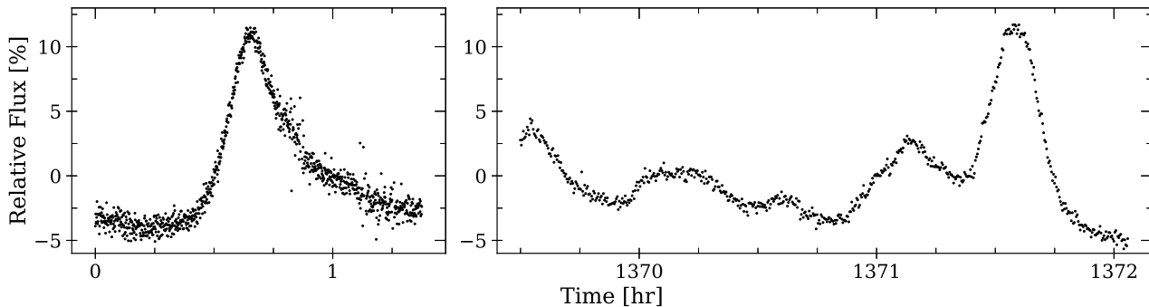
Figure 1. High-speed photometry taken with the 2.1 m Otto Struve telescope at McDonald Observatory, identifying pulsations on 2019 August 2 (left) and confirming them on 2019 September 29 (right) in the extremely low-mass white dwarf GD 278.
