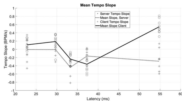
Fig. 8. Mean tempo slope across OWT latency.
