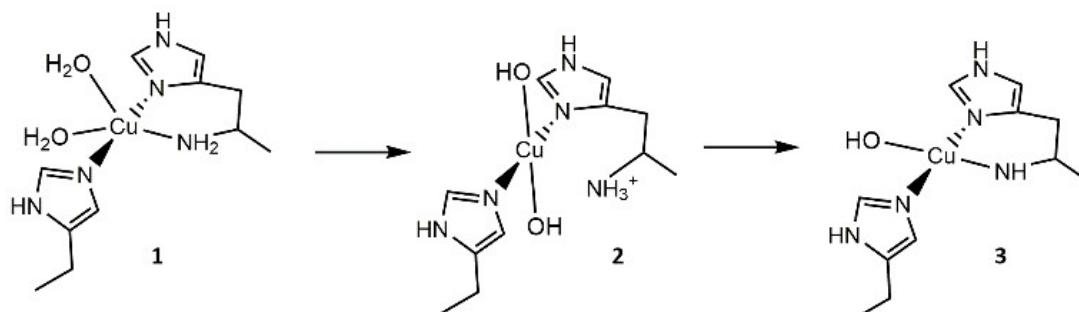
Figure 4. Hypothetical protonation states and coordination geometries of species 1, 2 and 3.
