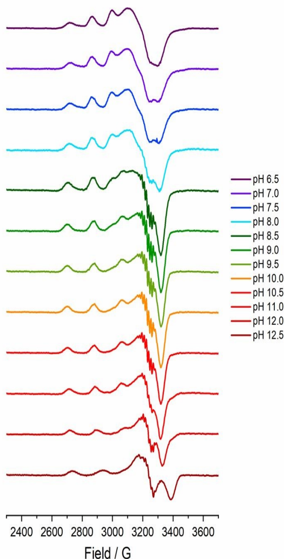
Figure 2. Frozen solution X-band EPR spectra (150 K) of B/(AA10) (0.4 mM) in a mixed buffer of MES, CHES, HEPES and CAPS (5 mM each) between pH 6.5 and 12.5.
