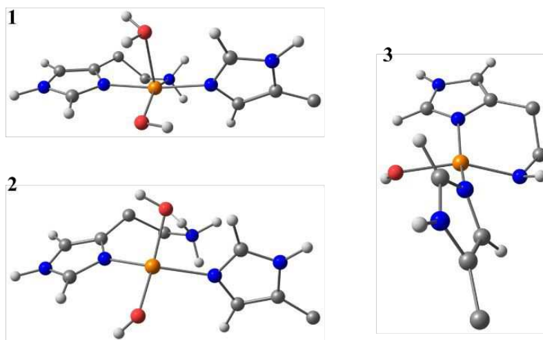
Figure 7. DFT optimised geometries of species 1, 2 and 3. Models are truncated, and certain atoms are hidden for clarity.
