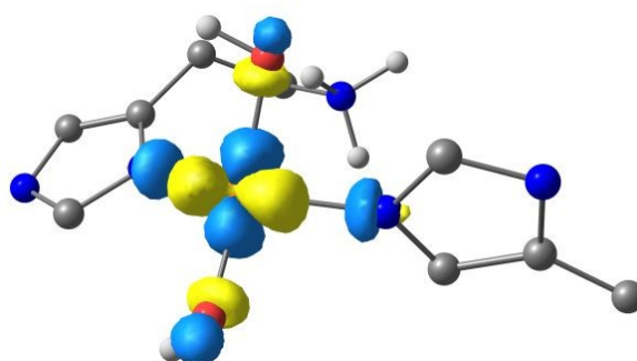
Figure 6. Hypothetical d(x^2-y^2) dominated SOMO of species 2 showing the orbital plane has rotated. (Colours denote orbital phase).
