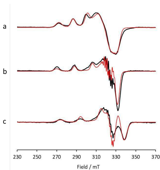
Figure 3. X-band EPR a) low pH species 1, with simulation (red), b) intermediate pH species 2, with simulation (red), c) high pH species 3, with simulation (red).
