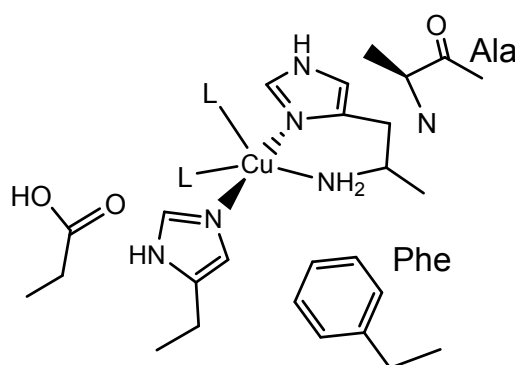
Figure 1. Active site of a chitin-active AA10 LPMO, depicting the histidine brace exogenous ligands (L) ligating to the Cu(II) ion, and conserved residues.
