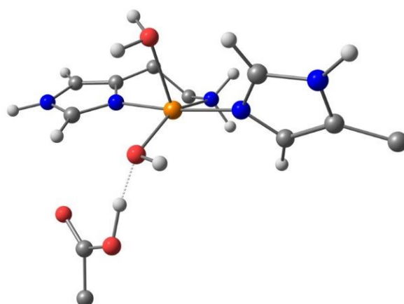
Figure 5. DFT model of species 1 (truncated for clarity) showing distorted square-pyramidal geometry and hydroxide/water coordination of exogenous ligands.
