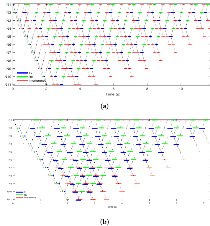
Figure 7. Simulated MAC schedules for the 2 km 10-hop scenario. Tx: Transmission, Rx: Reception. (a) LTDA-MAC [11]. (b) FD-LTDA-MAC.
