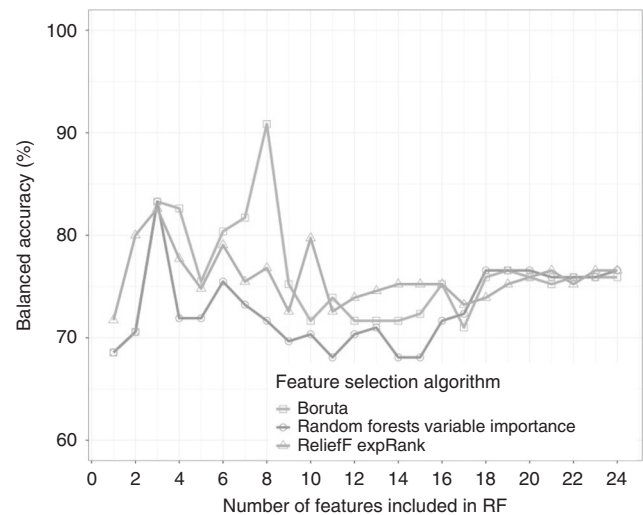
Fig. 3 Comparison of out-of-sample LOOCV balanced accuracy results of the random forests classifier using the features selected by each of the three feature selection algorithms.
