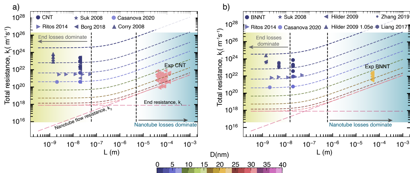
Fig. 5 Variation of the total resistance with nanotube length for a) CNTs and b) BNNTs. Most membrane simulations, with length in the order of nm, lie in the region of the plot where end resistance dominates, while experimental membranes lie in the region of the plot where nanotube flow resistance dominates. The lines for total resistance are generated using the HPW equation for k_1 and k_2 given in section 2.2, with L_s = 60 nm for CNTs and L_s = 10 nm for BNNTs.
