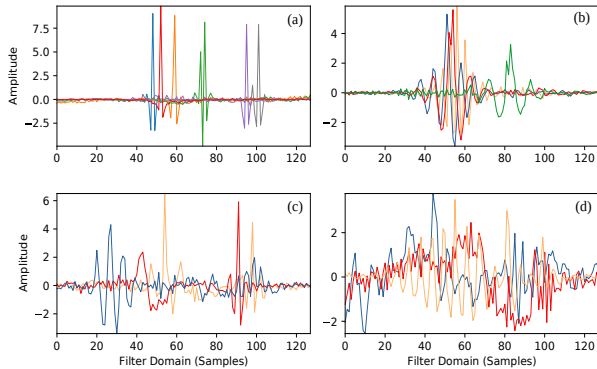
Figure 6: Shapes of the learned filters in ConvL1 fed with the raw magnitude spectrum (Fig. 4 (a)). (a) Sinc (short), (b) Sinc (medium support), (c) bimodal, (d) long-range correlation.
