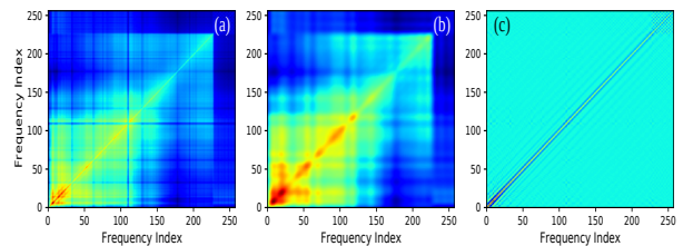
Figure 5: Covariance matrices computed using 300 signals of WSJ Eval-92. (a) Magnitude spectrum, (b) VT, (c) Exc.
