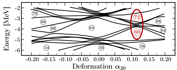
FIG. 4. Single proton energies as functions of the quadrupole deformation \alpha_{20} , calculated using the Woods-Saxon Hamiltonian. The numbers in the circles represent the numbers of protons that can fill the levels below the circles. Note a near-degeneracy of 6 levels at small prolate deformations, indicated with oval curve, cf. Nd–Hf evolution in Fig. 3
