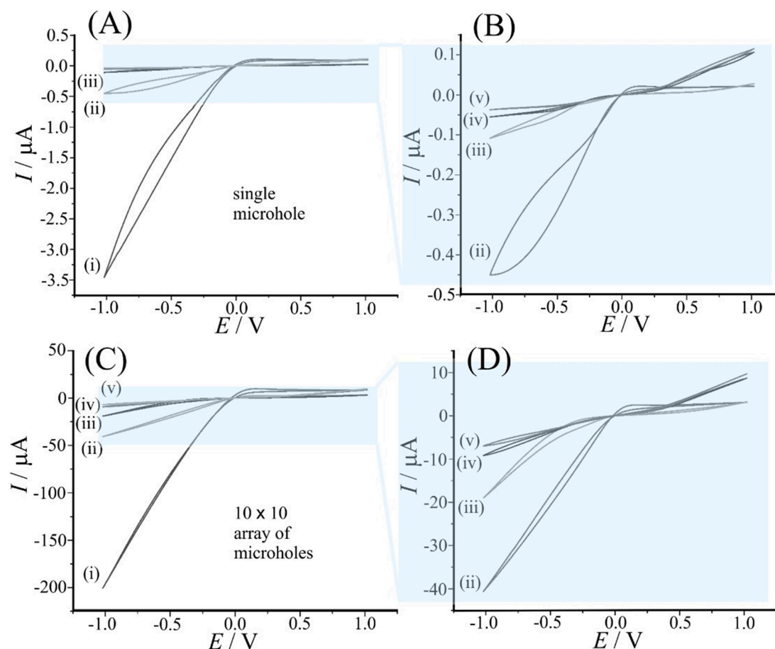
Fig. 2. (A,B) Cyclic voltammety data (scan rate 0.2 \text{ V s}^{-1} ) for a 10 \mu\text{m} microhole covered with PIM-EA-TB and immersed in aqueous 10 \text{ mM NaCl} at various pH values: (i) 2, (ii) 3, (iii) 4, (iv) 5, and (v) 6. (C,D) as before but for a 10 \times 10 array of microholes.
