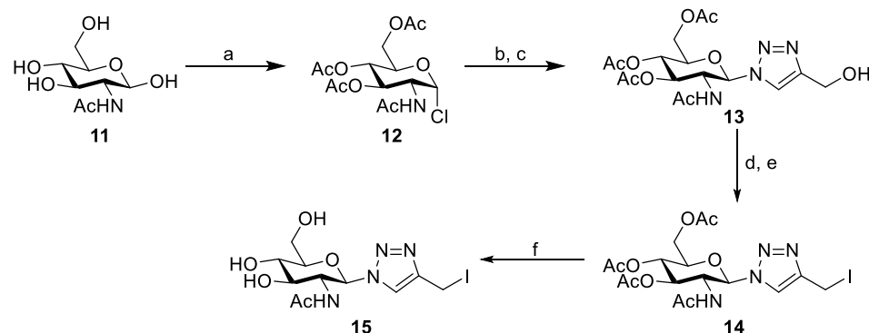
Scheme 3. Synthesis of GlcNAc iodomethyl-triazole; (a) \text{AcCl} , \text{CHCl}_3 , r.t., 16 h, 33%; (b) \text{NaN}_3 , TBAHS, \text{NaHCO}_3 (sat. aq.), DCM, r.t., 1 h, 96%; (c) propargyl alcohol, \text{Cu}(\text{MeCN})_4\cdot\text{BF}_4 , DCM/MeOH, r.t., 16 h, 95%; (d) \text{Ms}_2\text{O} , TEA, THF, 0^\circ\text{C} , 30 min; (e) NaI, acetone, 0^\circ\text{C} , 30 min, 97% (2 steps); (f) NaOMe (cat.), MeOH, r.t., 2 h, 53%.
