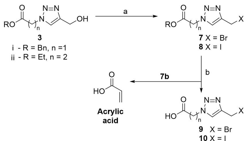
Scheme 2. Synthesis of bromomethyl- and iodomethyl-triazoles; (a) (i) \text{Ms}_2\text{O} , TEA, THF, 0^\circ\text{C} , 0.5 h; (ii) LiBr or NaI, THF, 0^\circ\text{C} , 0.5 h, 7a = 92%, 7b = 82%, 8a = 71%, 8b = 70% (2 steps); (b) LiOH (0.1 M, aq.)/THF (2:1), 5 h, 9a = 8%, 9b = 0%, 10a = 91%, 10b = 22%.
