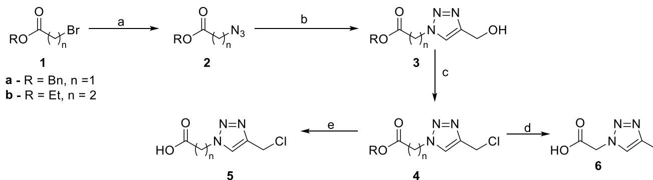
Scheme 1. Synthesis of malonyl and succinyl chloromethyl-triazoles; (a) NaN 3 (1 M in DMSO), r.t., 16 h, quant. yield; (b) propargyl alcohol, Cu(MeCN) 4 ·BF 4 , MeOH, r.t., 5–16 h, 73% ( 3a ), 71% ( 3b ); (c) SOCl 2 , CHCl 3 , r.t., 1 h, 85% ( 4a ), 92% ( 4b ); (d) Pd/C (2 mol%), Et 3 SiH (10 eq.), MeOH, 20 min, (71%); (e) HCl (3 M, aq.)/THF, 16 h, 50 °C, 85% ( 5a ), 85% ( 5b ).
