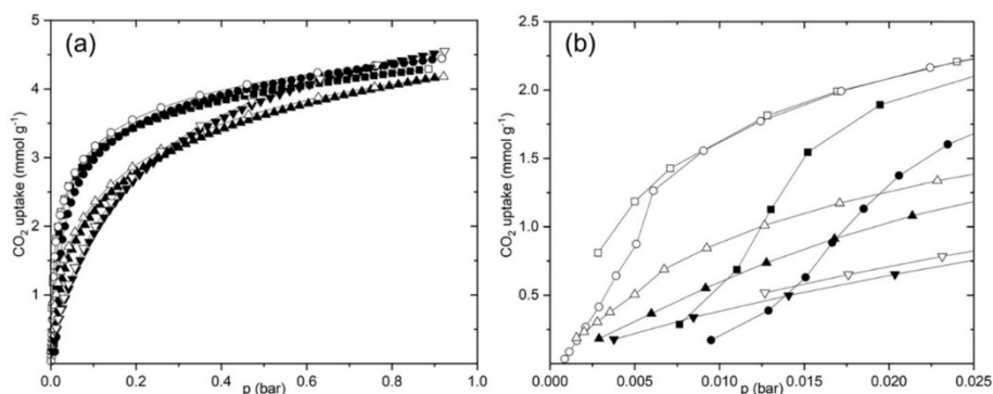
Figure 8. \text{CO}_2 isotherms at 298 K on \text{Na}_{9.8}\text{-Rho} (■), \text{Cu}_{1.0}\text{Na}_{7.8}\text{-Rho} (●), \text{Cu}_{3.4}\text{Na}_{3.0}\text{-Rho} (▲) and \text{Cu}_{4.9}\text{-Rho} (▼). Adsorption, closed symbols; desorption, open symbols.
