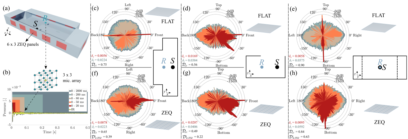
Figure 6. (a) Geometry of an ideal orchestra pit used in a 3D FDTD simulation. (b) Sample impulse response with different integration times used for the Spatial Decomposition Method (SDM). Spatio-temporal distributions of sound field energy ( 10 \log_{10} |p_s| ) for each coordinate plane in the orchestra pit received at location R from sound source S in (c–e) a pit with flat boundaries, and (f–h) a pit with sparsely distributed repetitions of equivalent surface impedance (ZEQ) patches.
