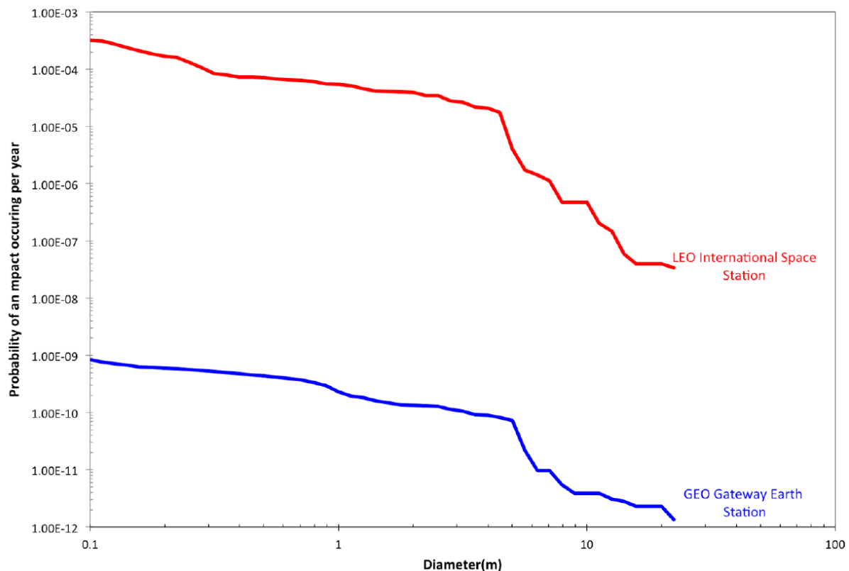
Fig 3. MIDAS predicted probability of an impact occurring per year vs diameter (logarithmic) of impactor for LEO and GEO stations [20].
