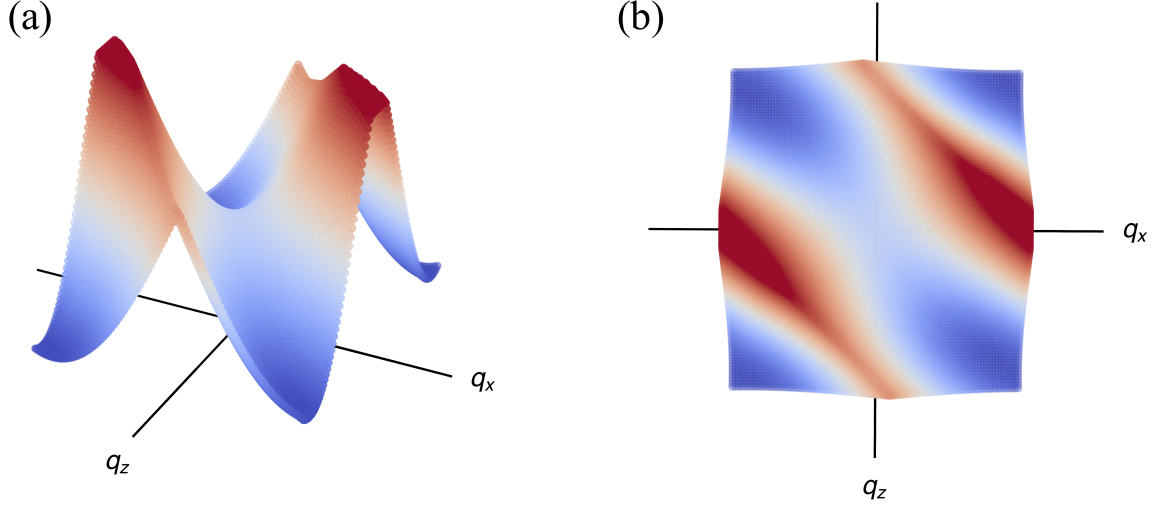
Figure 3. (a) Diagonal and (b) top view of the dispersion of the magnetic ground state within the (\mathbf{q}_x, \mathbf{q}_z) plane at 0 GPa. Red color highlights highest energies, while dark blue regions evidence energy minima.
