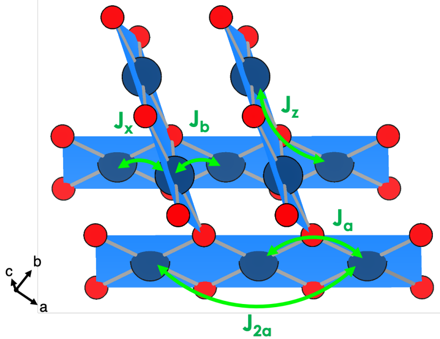
Figure 1. Magnetic exchange couplings considered in this study. The different interactions are highlighted by green arrows. Blue and red spheres indicate copper and oxygen atoms, respectively. Square planar environments are represented in blue.
