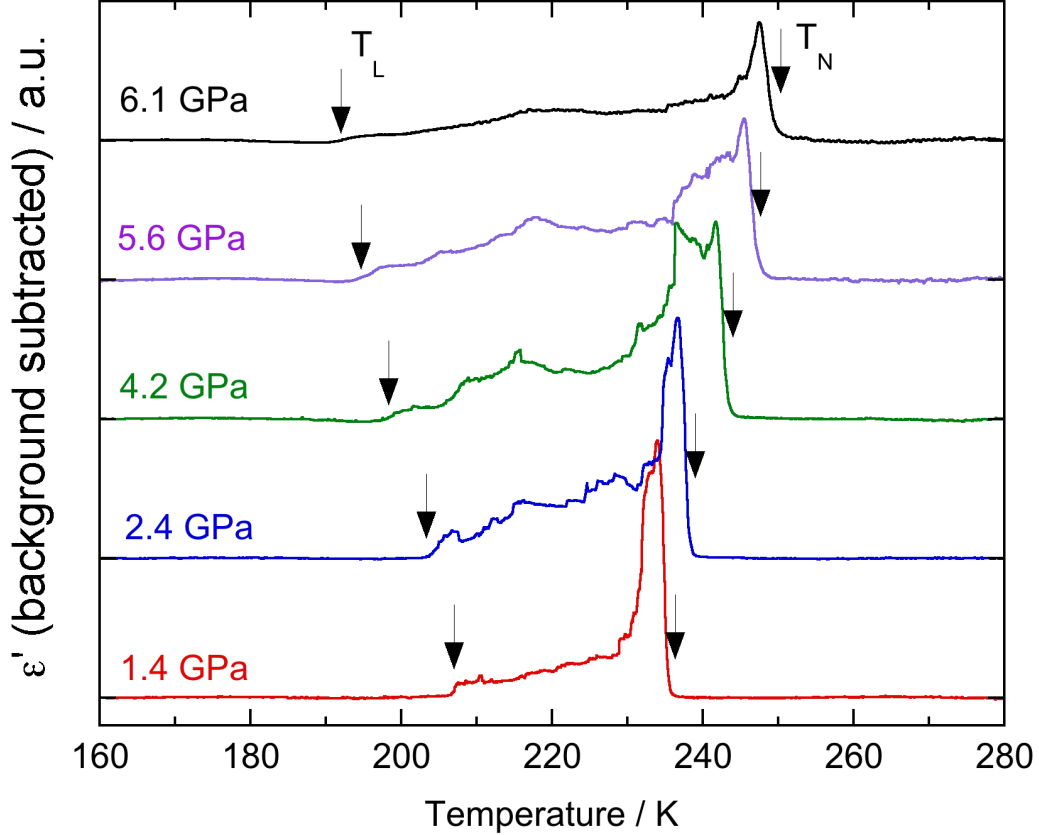
Figure 6. Zoom of the dielectric constant curves shown in Figure 5 after subtraction of an arbitrary polynomial background to reveal T_N and T_L transitions evidenced by arrows. Curves have been shifted for clarity.
