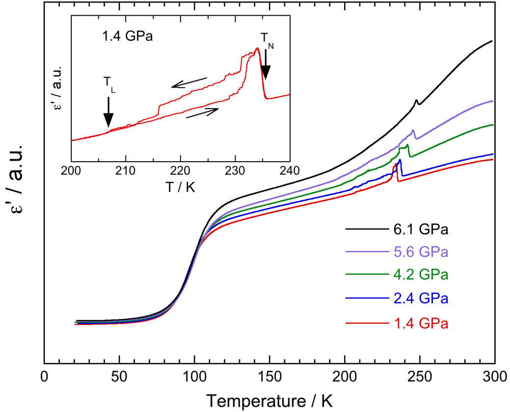
Figure 5. Dielectric constant curves of single crystal CuO for \mathbf{E} // \mathbf{b} from high pressure capacitance measurements with increasing temperature. The inset shows the region of the two magnetic phase transitions for 1.4 GPa, indicated by the arrows. The upper transition ( T_N ) appears as a sharp step reproducible on warming and cooling. The lower transition ( T_L ) appears as a much smaller anomaly. The region between T_L and T_N shows marked hysteresis between the cooling and warming cycles, with irreproducible behaviour on cooling.
