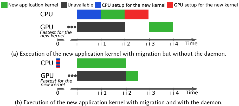
Fig. 5. Execution without and with a daemon that sets up OpenCL and/or CUDA in advance. With the daemon the new application kernel does not spend time in setup code when it migrates. The daemon performs the setup once when it starts as indicated by the striped bar at time zero in (5b). Data transfers are not shown for simplicity.
