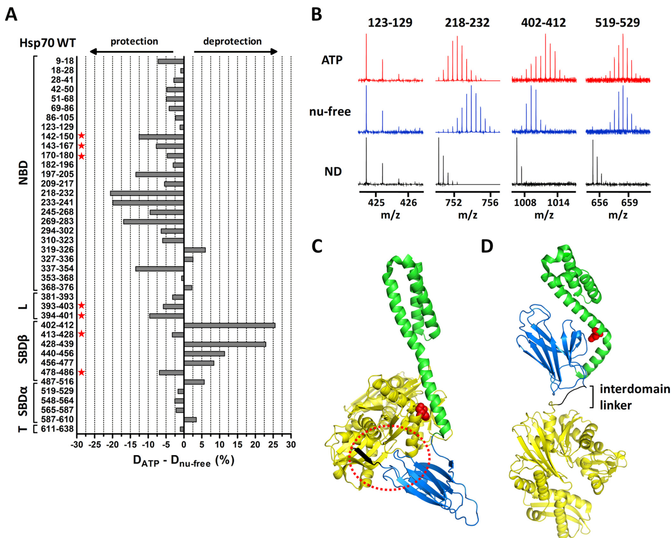
FIG. 4. ATP-induced allosteric domain docking of Hsp70. A , deuteriation level differences of Hsp70 peptides in ATP-bound and nucleotide-free state after 1 h of incubation in deuterated buffer. Numbers at left indicate the Hsp70 peptide fragments; schematic representation at left shows Hsp70 domain constitution; L , interdomain linker; T , C-terminal tail. B , original mass spectra of representative peptide fragments of Hsp70 incubated in non-deuterated buffer (ND) or for 1 h in deuterated buffer in the presence/absence of ATP. C and D , crystal structures of Hsp70 bacterial homologue DnaK in ATP-bound state ( C , PDB code 4jne) and in nucleotide-free/ADP state ( D , PDB code 2kho). NBD, interdomain linker, SBD \beta , and SBD \alpha are shown in yellow, black, marine, and green, respectively. Encircled region ( C ) shows tight association of IA subdomain of NBD, linker, and SBD loops L_{2,3}/L_{6,7} (peptides indicated with a star in A ) when SBD \beta is docked onto NBD (compare with I164D mutant, Fig. 5A). Residues I160 and D526 (human numbering I164 and D529) are highlighted in red in ATP/ADP structures, respectively. The images were created in PyMOL.
