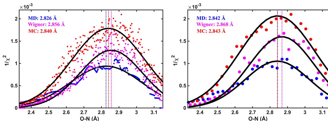
Figure 3. The inverse of the \chi^2 fitting errors plotted as a function of the O-N interatomic distance and fits as described in the text with bin widths of 0.1% (left) and 1% (right) of the O-N distance of the ground state structure as bin size, respectively. Blue (MD pool), purple (Wigner pool) and red (MC pool) dots: best-fitting structure with the highest 1/\chi_i^2 value retained in each distance bin, for the experimentally measured time delay of 3.55 ps of NMM. Black curves: fits using Gaussian functions. The maxima are taken as the determined molecular structure.
