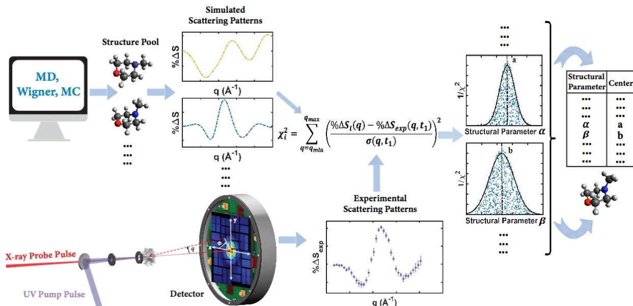
Figure 2. Concept of the method for determining molecular structures in excited electronic states from experimental scattering patterns.
