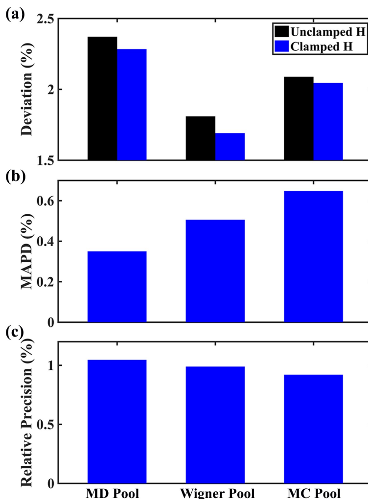
Figure 6. Comparison of structure analysis results using three different structure pools. (a) The scattering pattern deviations calculated as \frac{\sum_q |\% \Delta S_{exp} - \% \Delta S_{theory}|}{\sum_q 1} and averaged over all 25 time points, where \% \Delta S_{exp} is the experimental scattering pattern at each time point (black dots in Figure 5) and \% \Delta S_{theory} is the corresponding calculated pattern (red curve in Figure 5). Black and Blue bars: Results when using structural pools before (black) and after (blue) clamping the C-H bond lengths, respectively. (b) Mean absolute percent deviation calculated by Equation 4 with the determined structural parameters as r'_{ij} and distances of representative structure as r''_{ij} . (c) Averaged relative experimental precision over 21 interatomic distances as reported in Table 1 for analyses using the individual structure pools.
