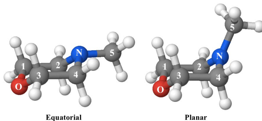
Figure 1. The equatorial and planar structures of NMM.
