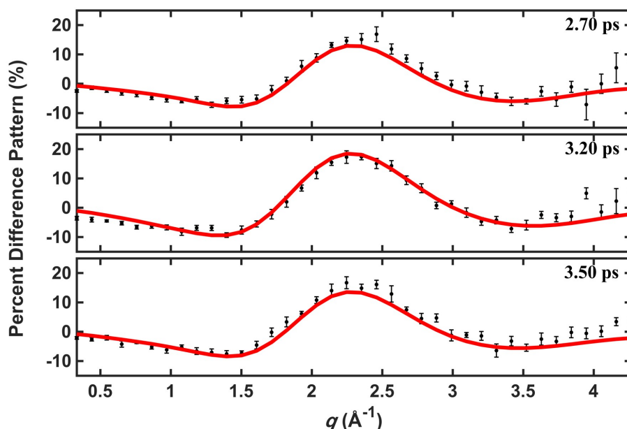
Figure 5. Experimental and calculated percent difference scattering patterns at several representative delay time points. The experimental results (black dots) are adopted from Ref 14 with 3\sigma error bars and scaled to 100% excitation. Calculated scattering patterns (red lines) are computed using the structural parameters determined with the present method, using the Wigner pool and a computed electronic correction term as described in the text.
