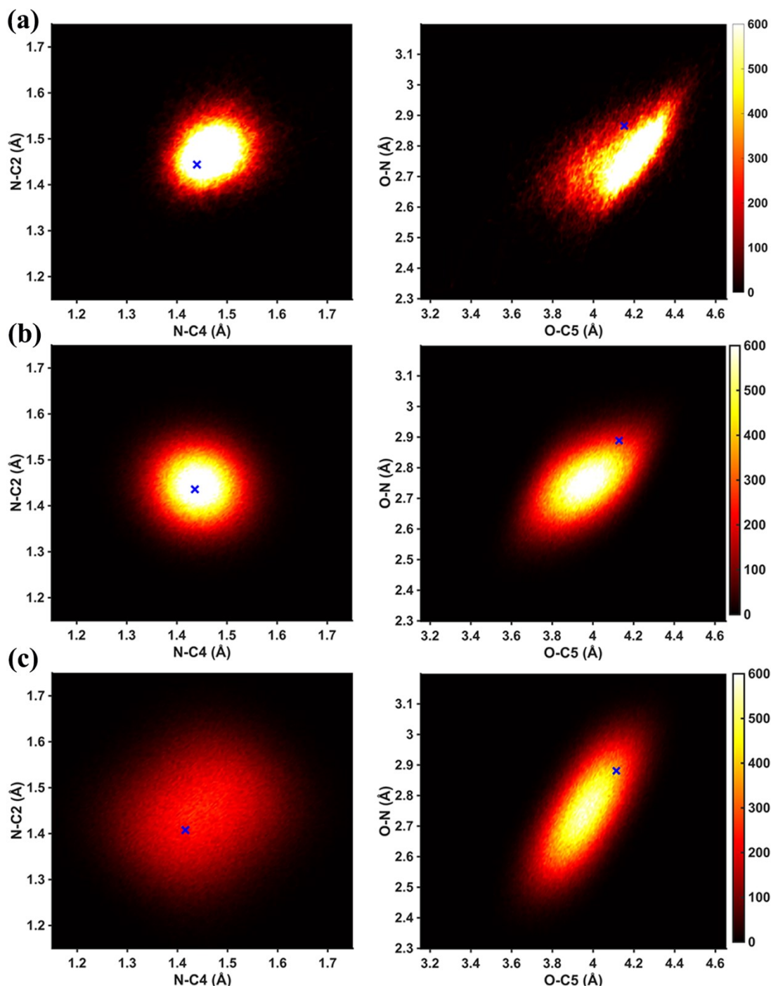
Figure 7. Phase space density of three structural pools, projected onto two of the structure dimensions. (a) MD pool. (b) Wigner pool. (c) MC pool. The color intensity shows the number of structures per pixel in each structure pool. A pixel is defined as 0.004 \times 0.004 \text{ \AA}^2 for the left column and 0.008 \times 0.008 \text{ \AA}^2 for the right column. Blue crosses: best-fitting structural parameters determined using each individual structure pool.
