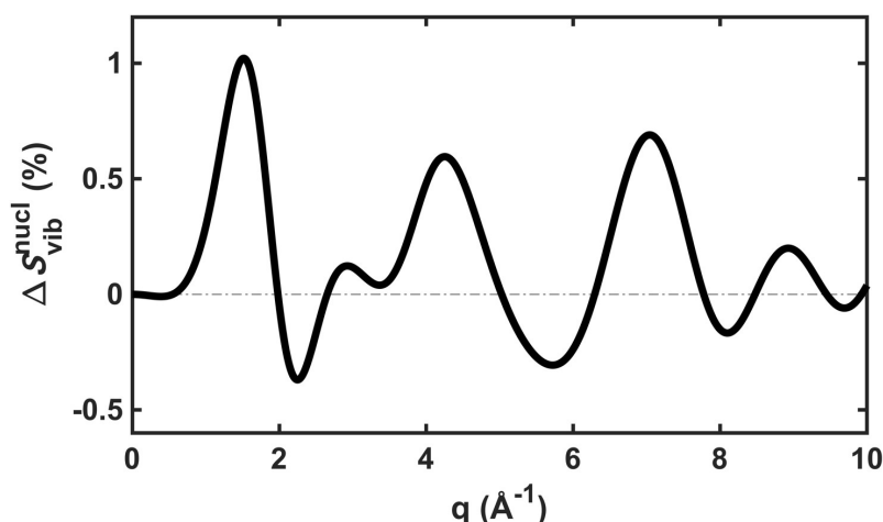
Figure 4. The vibrational correction term, \Delta S_{\text{vib}}^{\text{nucl}}(q, \mathbf{R}') , for NMM in the 3s Rydberg state, assuming a vibrational temperature of 1000 K.
