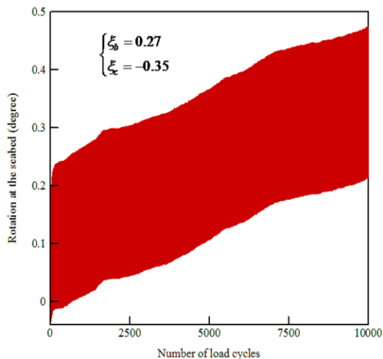
Fig.11 Computed pile rotation occurs when piles are placed in a dry medium-dense sand and are subjected to sinusoidal loading.
