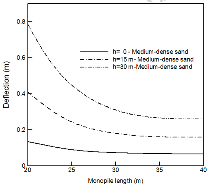
Fig. 8 Dependence of pile head deflection on pile length at 20 MN
