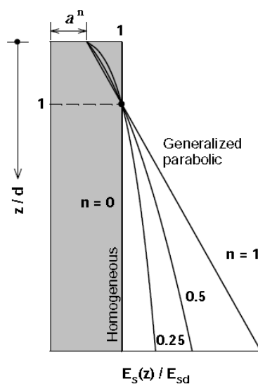
Fig. 19 The OWT model which was adopted to account for impedance functions
