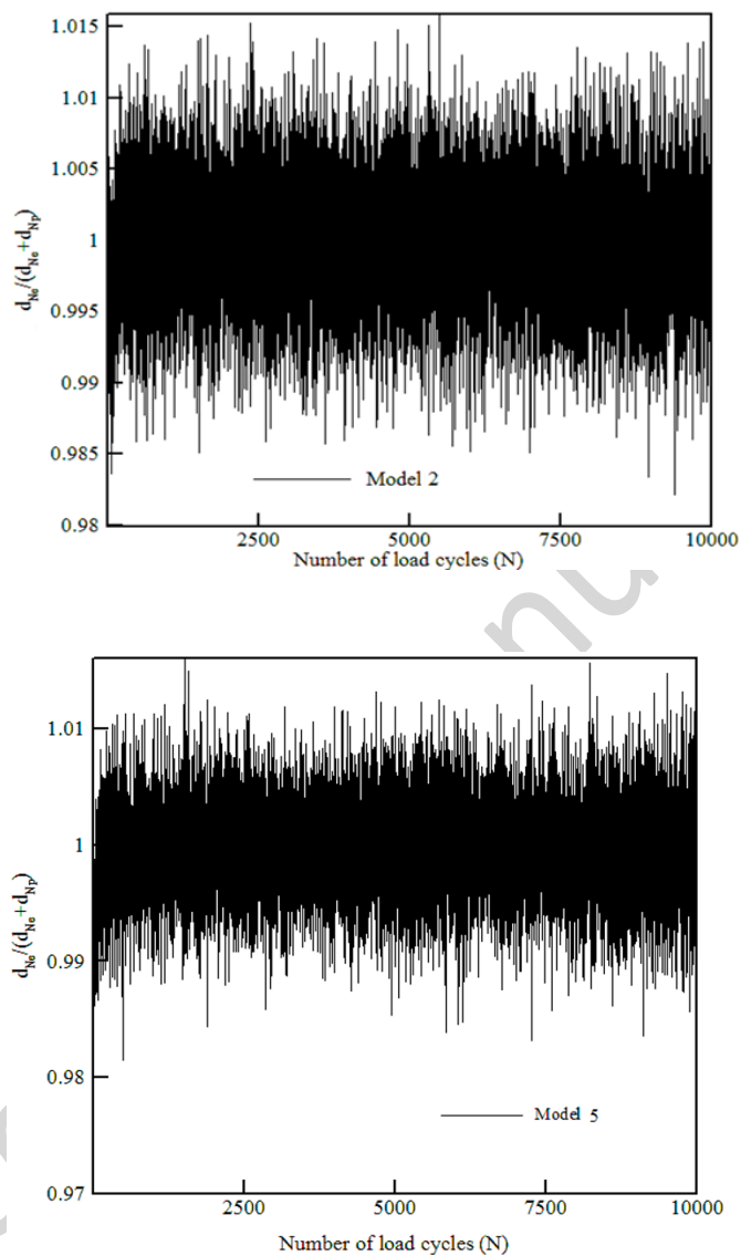
Fig. 17 Ratio of elastic displacement to total displacement in long-term cycling (dry analysis)
