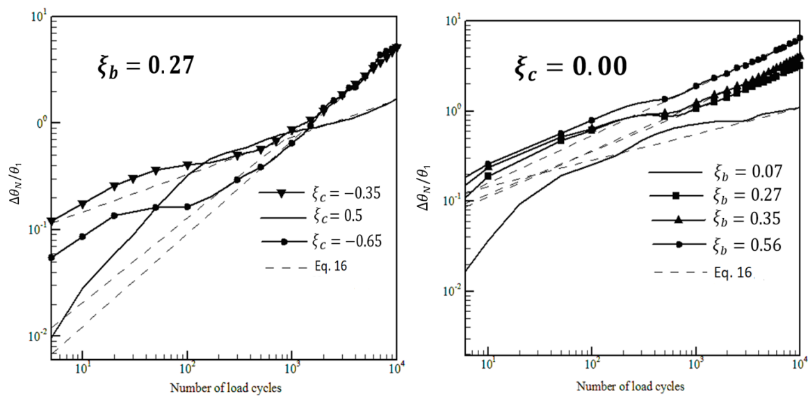
Fig.14 Normalized accumulated rotation as a function of the number of cycles (in partially drained sand). Dotted lines represents Eq.16
