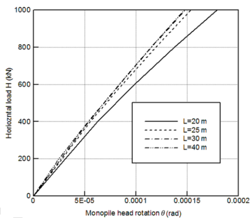
Fig. 22 Resultant monopile head rotation versus acting horizontal load for various aspect ratios.
