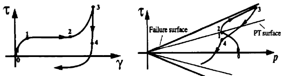
Fig. 5 A typical shear stress-strain response and corresponding effective stress path (Para 1996, Yang 2000)
