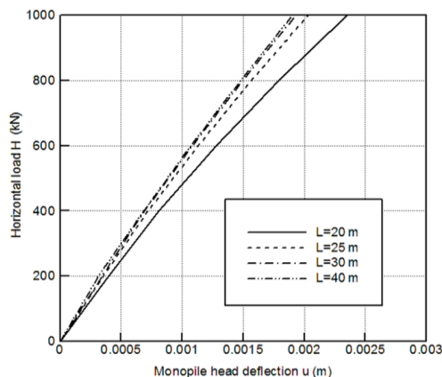
Fig. 21 Monopile head displacement versus applied horizontal load for various aspect ratios.
