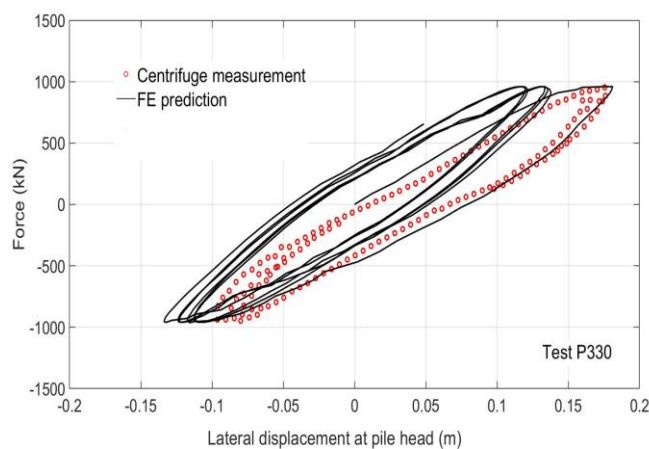
Fig. 3.2 Numerically computed and experimentally measured force-displacement curves at pile head in P330 event
