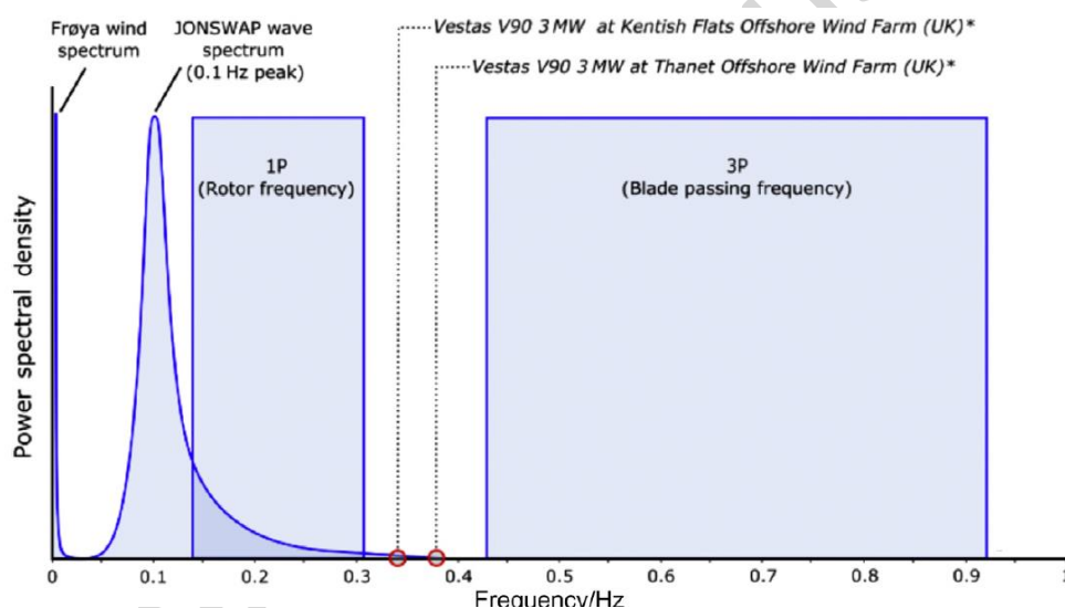
Fig.2 A power spectral density plot which presents the forcing frequency distribution for a typical three-bladed Vestas V90 3 MW OWT (Lopez-Querol et al. 2017)
