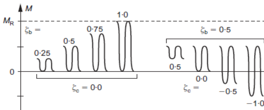
Fig. 9 Characteristics of cyclic loading defined in terms of \xi_b and \xi_c .
