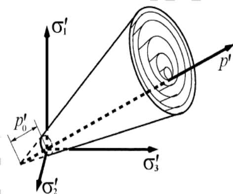
Fig. 4.1 Yield envelopes in principal stress space ( p' : mean effective stress)
