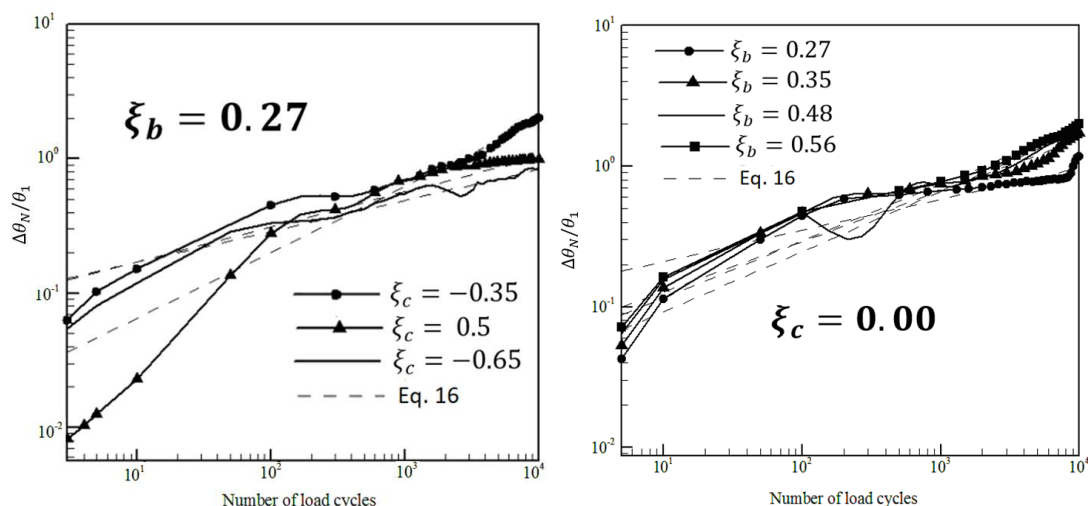
Fig. 13 Normalized accumulated rotation as a function of number of cycles (in a drained analysis).
