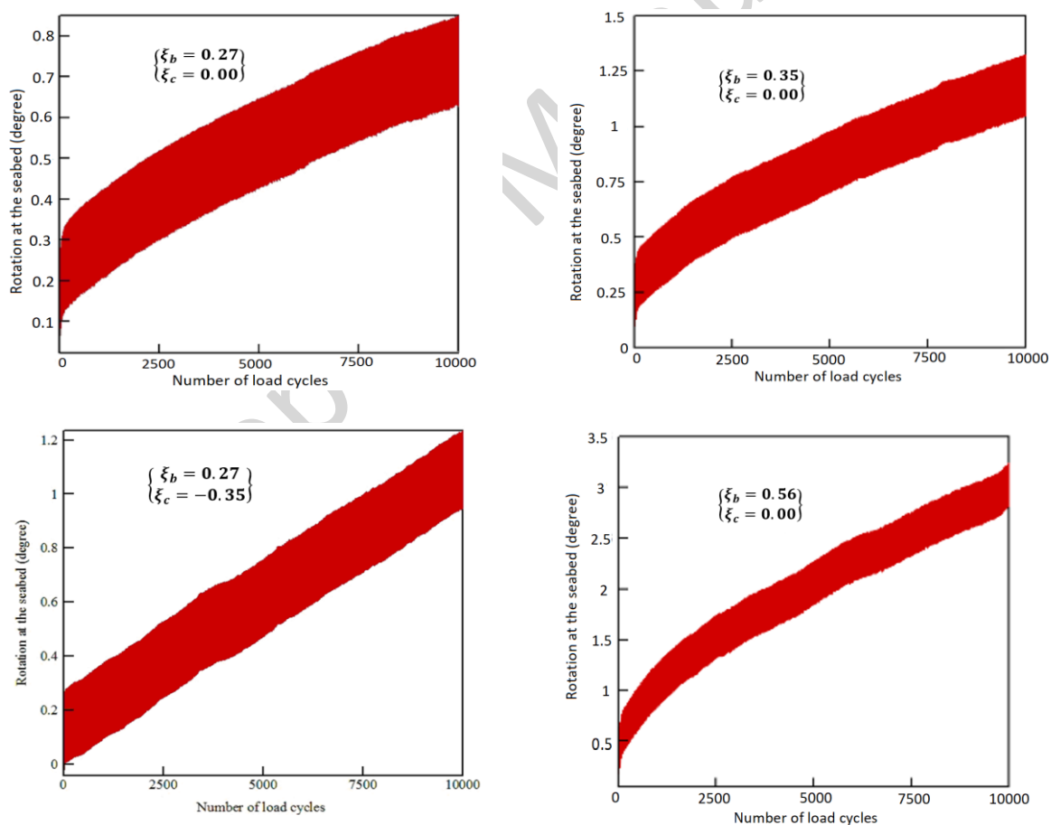
Fig.11 Computed pile rotation occurs when piles are placed in a dry medium-dense sand and are subjected to sinusoidal loading.
