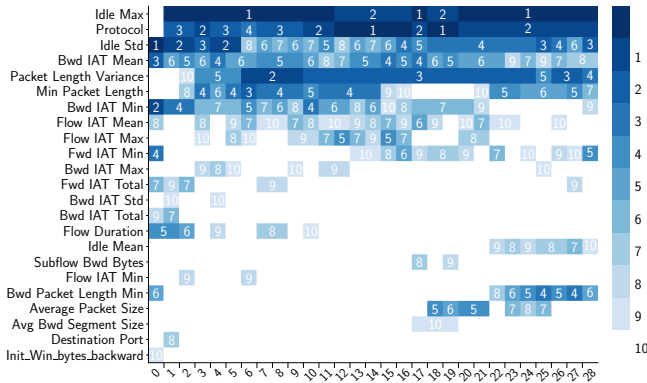
Figure 8: Feature ranking map of the DNN model learned with INSOMNIA at \sigma = 50\% . We plot the rank (1–10) of the features (axis Y), which are ranked in the top ten positions of the feature ranking determined with DALEX along the consecutive windows (axis X) processed over time. Window 0 covers the traces processed in initialization phase. Windows 1–28 cover the traces processed in the incremental phase.
