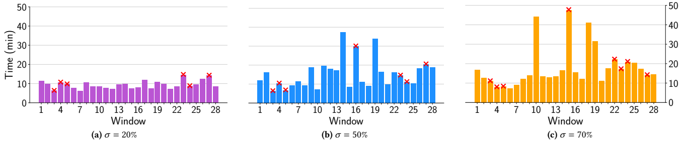
Figure 5: Computation time (in minutes) spent completing the incremental learning phase of INSOMNIA for varying \sigma at 20%, 50%, and 70%. Crosses (X) indicate latency periods for which the fine-tuning of the DNN model completes after all traces in the current window have been acquired.
