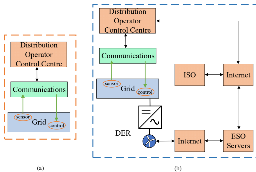
Figure 23. (a) Traditional control communications compared to (b) AC/DC hybrid grid communications.
