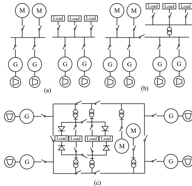
Figure 1. Traditional AC ship distribution systems: (a) propulsion isolated, (b) radial IPS, (c) modern AC zonal distribution system.
