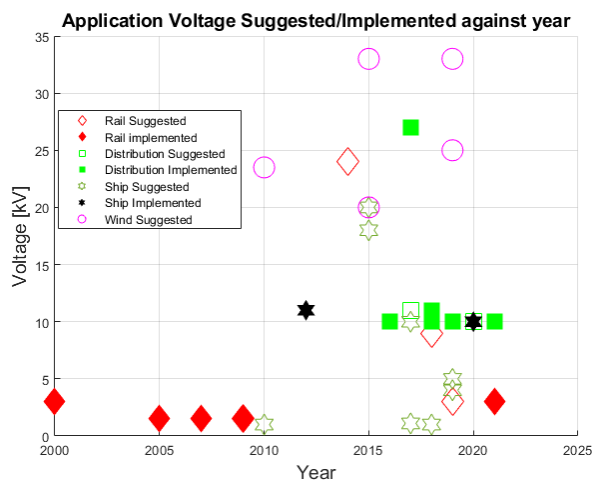
Figure 6. Suggested and implemented application voltage level.
