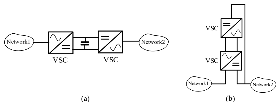
Figure 7. (a) B2B soft-open point configuration. (b) Soft-power bridge.
