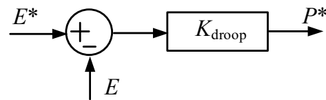
Figure 22. Voltage droop control.
