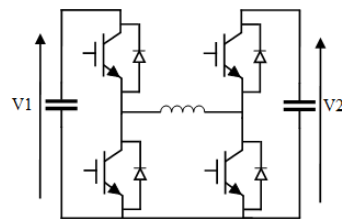
Figure 14. Buck-boost.
