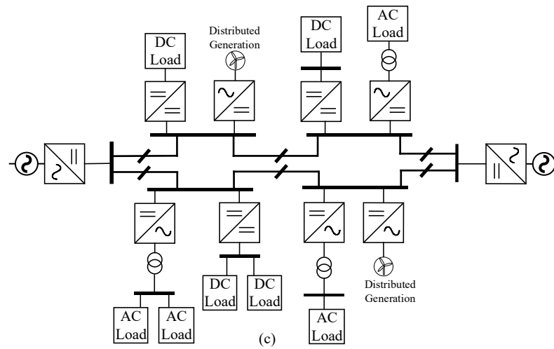
Figure 8. Network topologies: (a) radial, (b) hand-in-hand multiterminal, and (c) ring.
