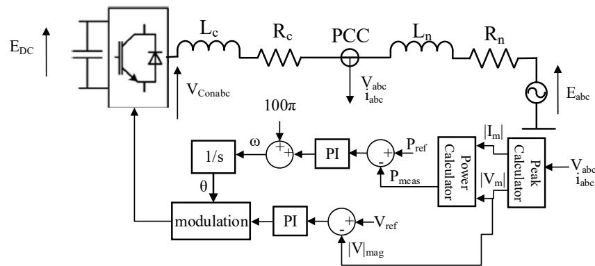
Figure 21. Virtual synchronous machine general control.
