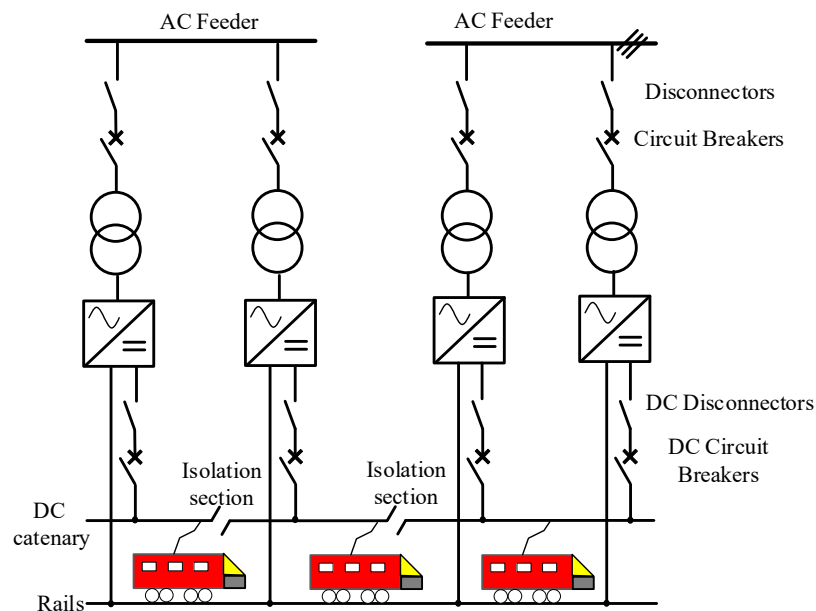
Figure 3. DC rail distribution system.
