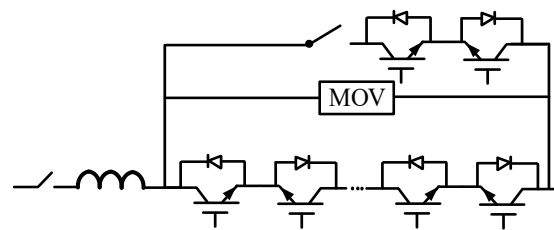
Figure 19. Hybrid DC circuit breaker.
