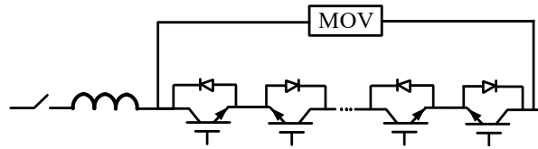
Figure 18. Solid-state DC circuit breaker.
