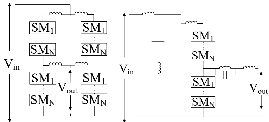
Figure 17. Push–pull and tuned filter MMDC.
