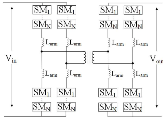
Figure 16. Dual active bridge modular multilevel converter.
