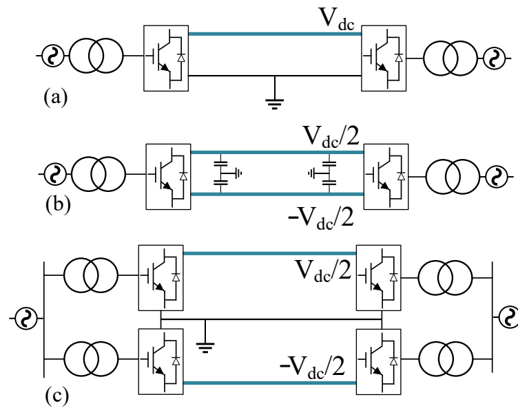
Figure 9. MVDC bus structures. (a) Unipolar asymmetric. (b) Unipolar symmetric. (c) Bipolar.
