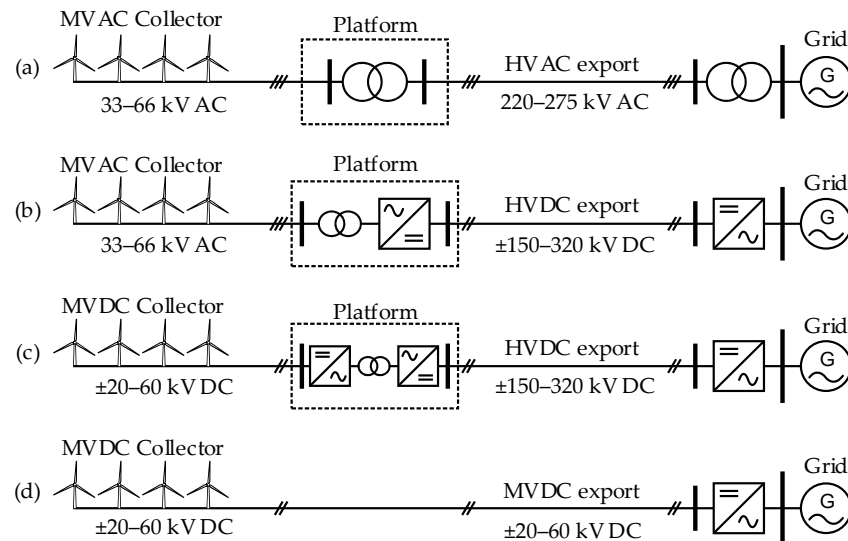
Figure 4. Connection options for offshore wind farms: (a) MVAC collector with HVAC export, (b) MVAC collector with HVDC export, (c) MVDC collector with HVDC export, and (d) MVDC collector and export. Indicative voltage levels are based on existing AC wind farms [69] and proposed DC wind farm designs [65,68].
