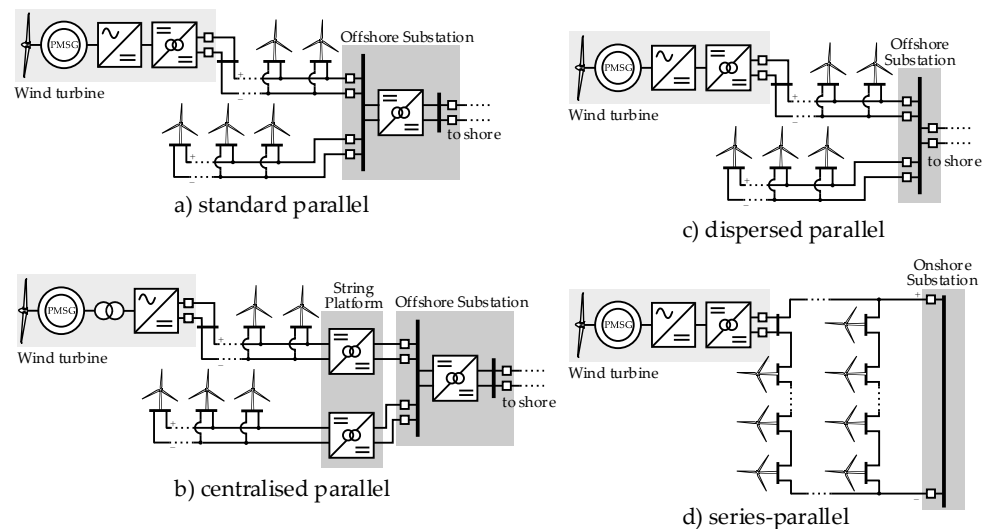
Figure 5. DC collection system options: (a) standard parallel, (b) centralised parallel, (c) dispersed parallel, (d) series-parallel
