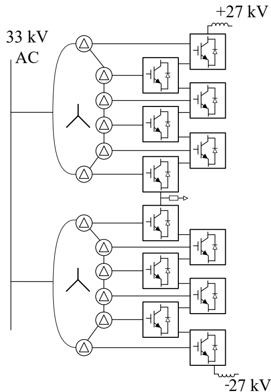
Figure 13. Converter station configuration of Angle-DC Project.
