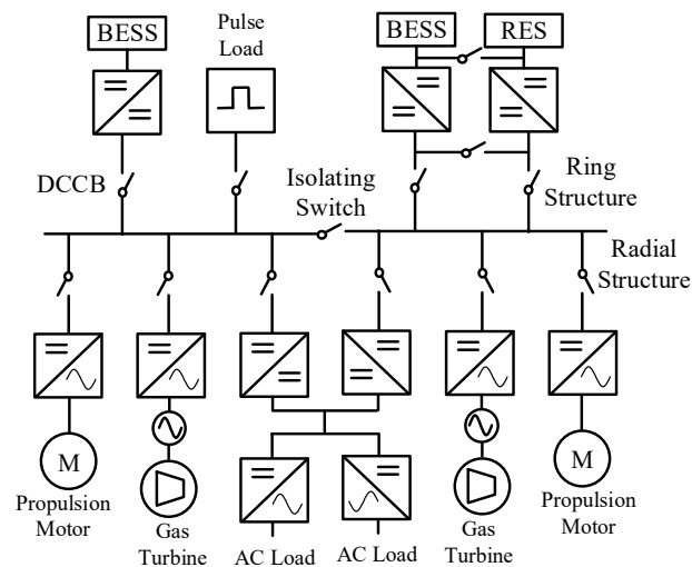
Figure 2. Generic DC shipboard IPS.
