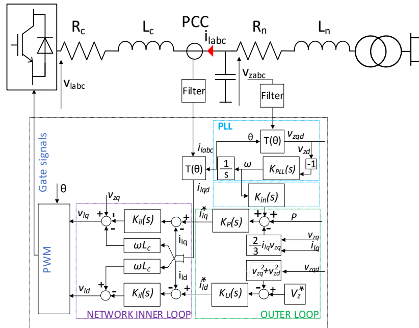
Figure 20. Traditional current control.
