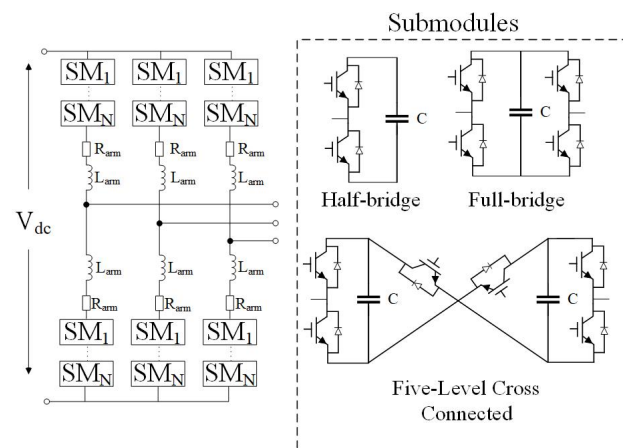
Figure 12. MMC and submodules.
