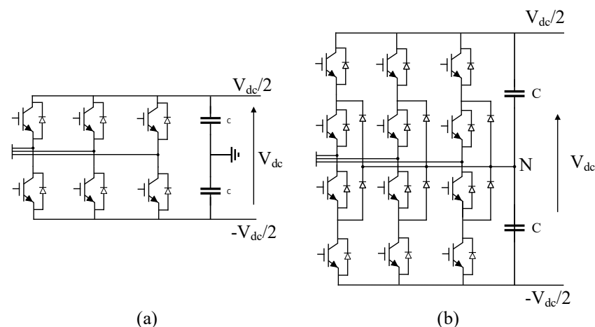
Figure 11. (a) Two-level converter (2L). (b) Three-level neutral-point clamped converter (3L-NPC).
