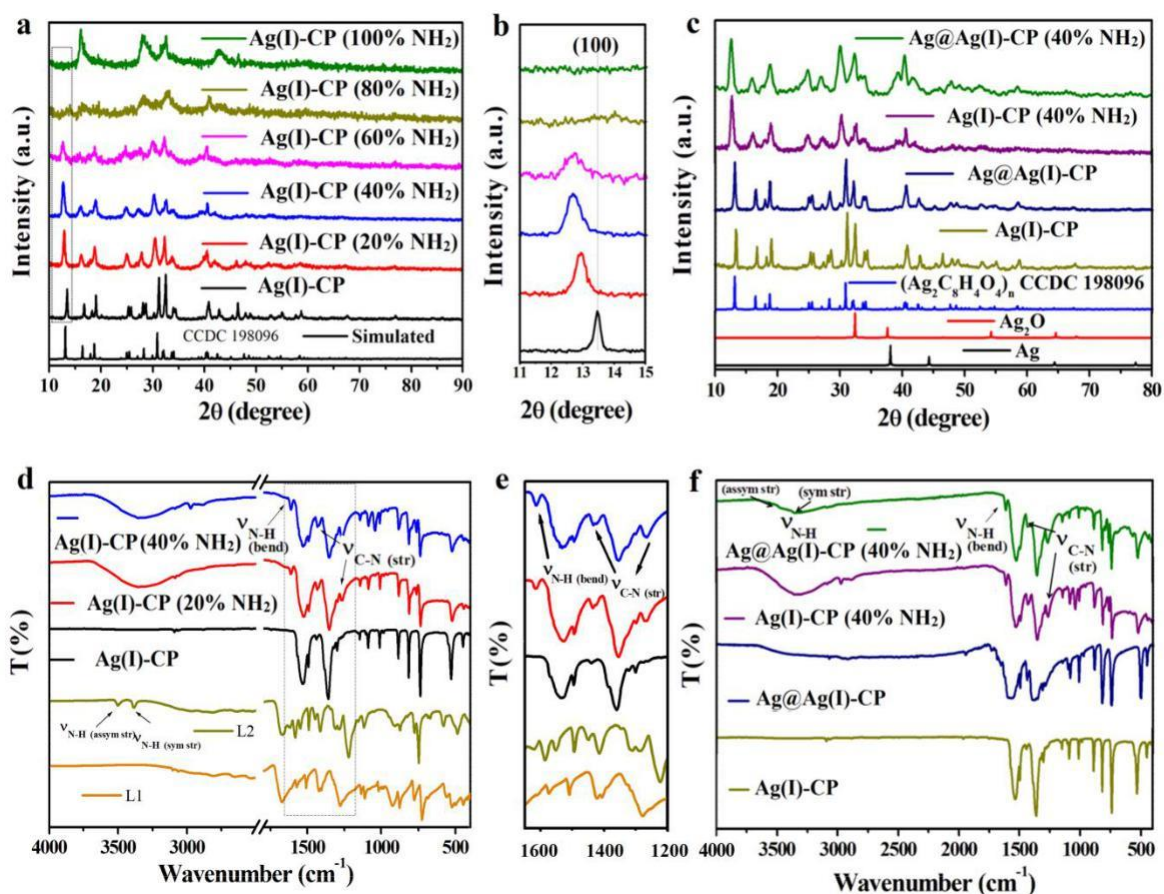
Fig. 1. (a) PXR patterns and (b) high-resolution XRD patterns of the selected area ( 11^{\circ} - 15^{\circ} ) of the mixed ligand CPs with their parent species, and (c) comparison of the PXR patterns with Ag@Ag(I)-CP (40% NH 2 ), and Ag@Ag(I)-CP. (d-e) FTIR spectra of mixed ligand CPs with their parent species, L1, and L2 at (d) 4000-400 cm -1 , and (e) 1650-1200 cm -1 , and (f) comparison of FTIR spectra with Ag@Ag(I)-CP (40% NH 2 ), and Ag@Ag(I)-CP.
