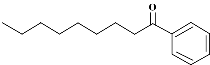
Nonanophenone
