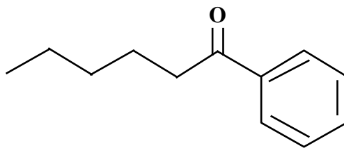
Butyrophenone
