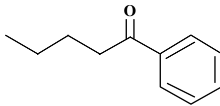
Valerophenone
