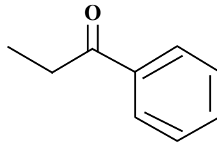
Propiophenone
