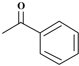
Acetophenone
