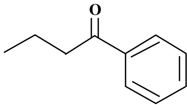
Butyrophenone
