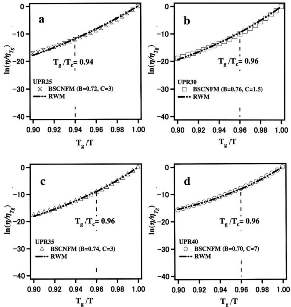
Fig. 1. Temperature dependence of the viscosity described by Eqs. (6), (BSCNFM) and Eqs. (9) and (10), (RWM) for UPR25 (a), UPR30 (b), UPR35 (c) and UPR40 (d).
