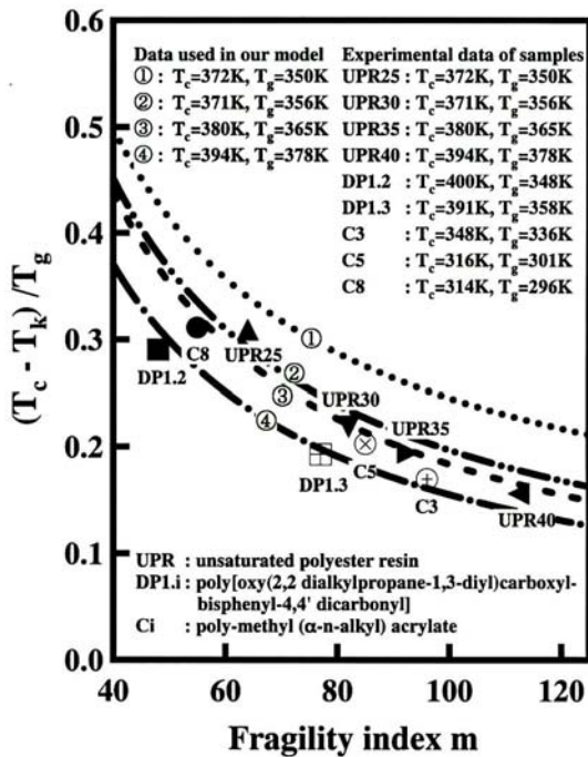
Fig. 2. The relationship between the normalized temperature range of cooperativity and the fragility index for three sample families of polymeric materials. The numbers after the name of the chemical compound represent the styrene content (in %W/W), the number of carbon atoms in the lateral chain and the number of carbon atoms of the side chain attached to the tertiary carbon of the propyl spacer for UPR, C and DP1, respectively.
